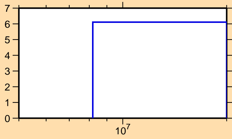
\Delta\sigma/\sigma vs. E for ^{131}\text{Cs}(n,\text{inel.})
