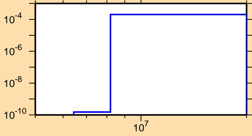
\sigma vs. E for ^{131}\text{Cs}(n,n\alpha)
