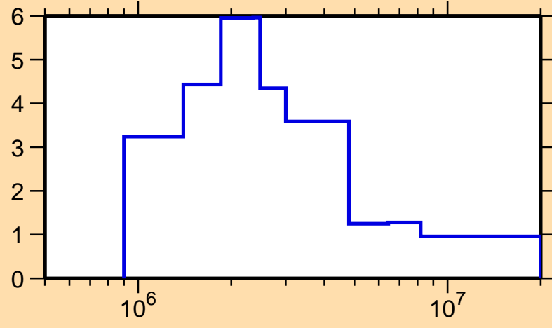
\Delta\sigma/\sigma vs. E for ^{131}\text{Cs}(n, tot.)
