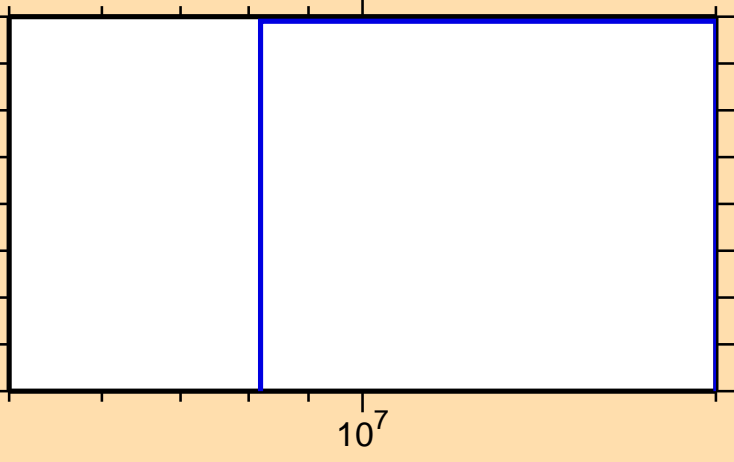
\sigma vs. E for ^{131}\text{Cs}(n,t)
