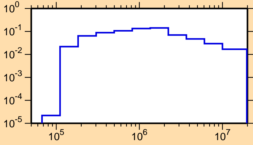
\sigma vs. E for ^{132}\text{Cs}(n,n_2)
