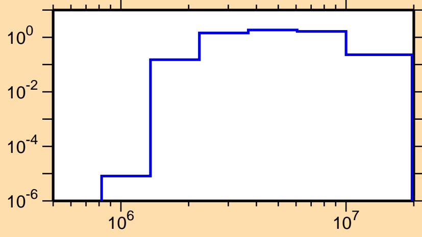
\sigma vs. E for ^{132}\text{Cs}(n,n\text{cont.})
