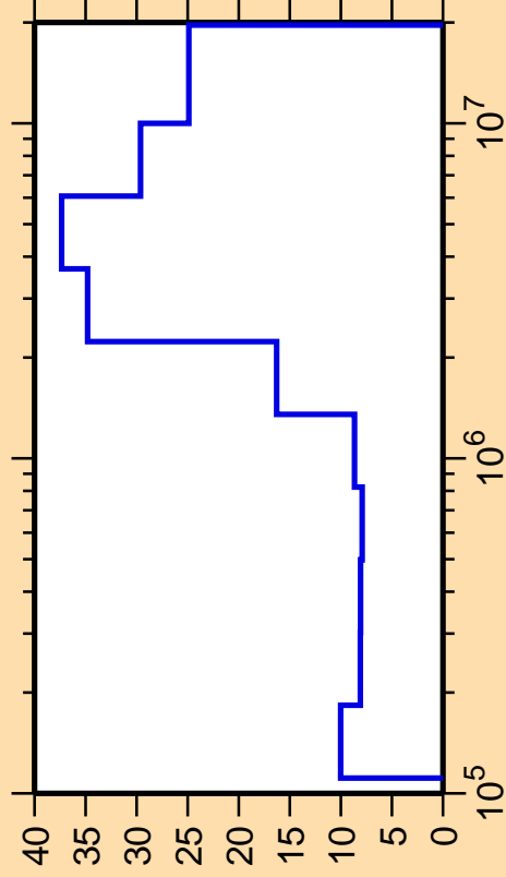
\Delta\sigma/\sigma vs. E for ^{132}\text{Cs}(n,n_4)
