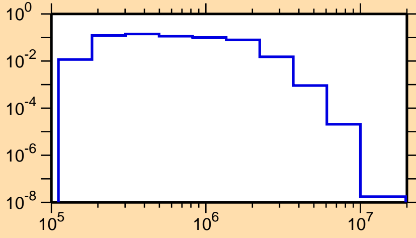
\sigma vs. E for ^{132}\text{Cs}(n,n_4)
