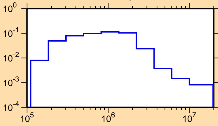
\sigma vs. E for ^{132}\text{Cs}(n,n_3)
