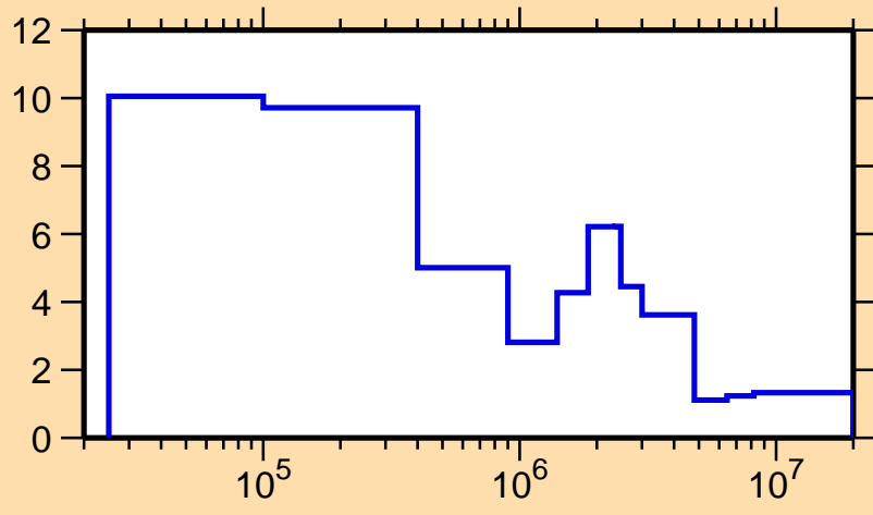
\Delta\sigma/\sigma vs. E for ^{132}\text{Cs}(n, \text{tot.})
