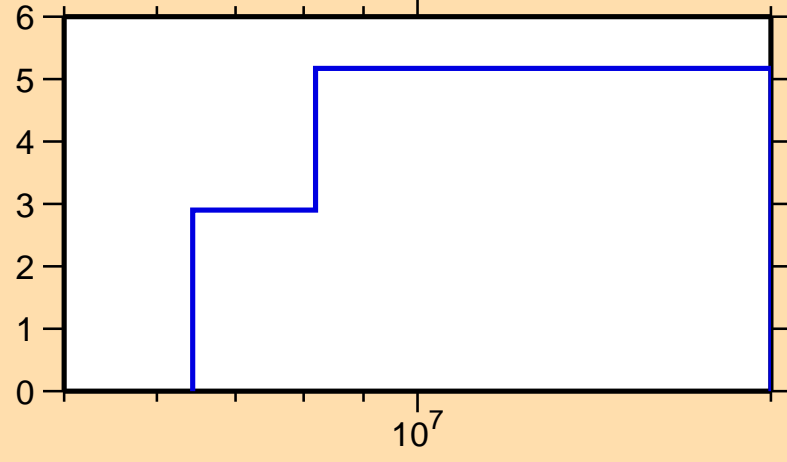
\Delta\sigma/\sigma vs. E for ^{132}\text{Cs}(n,\text{inel.})
