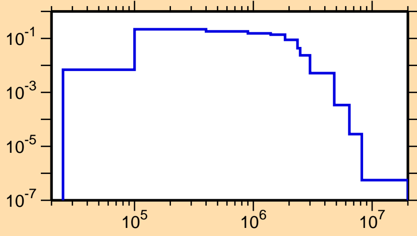
\sigma vs. E for ^{132}\text{Cs}(n,n_1)
