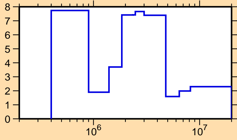
\Delta\sigma/\sigma vs. E for ^{132}\text{Cs}(n, \text{el.})
