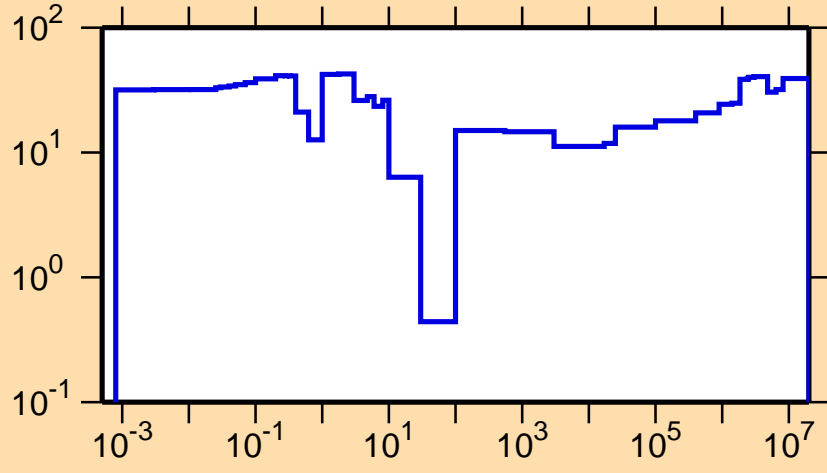
\Delta\sigma/\sigma vs. E for ^{132}\text{Cs}(n,\gamma)
