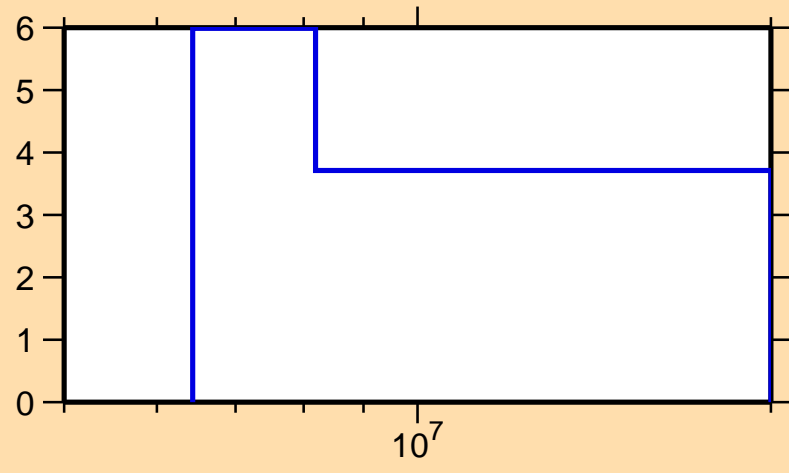
\Delta\sigma/\sigma vs. E for ^{132}\text{Cs}(n,2n)
