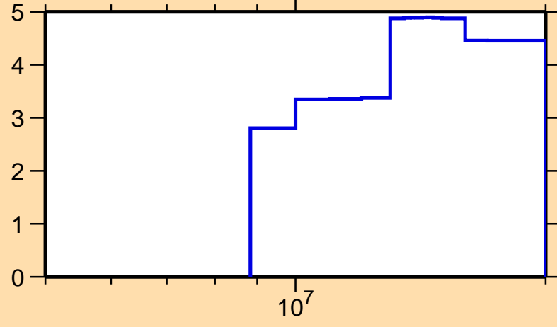
\Delta\sigma/\sigma vs. E for ^{133}\text{Cs}(n,\text{inel.})
