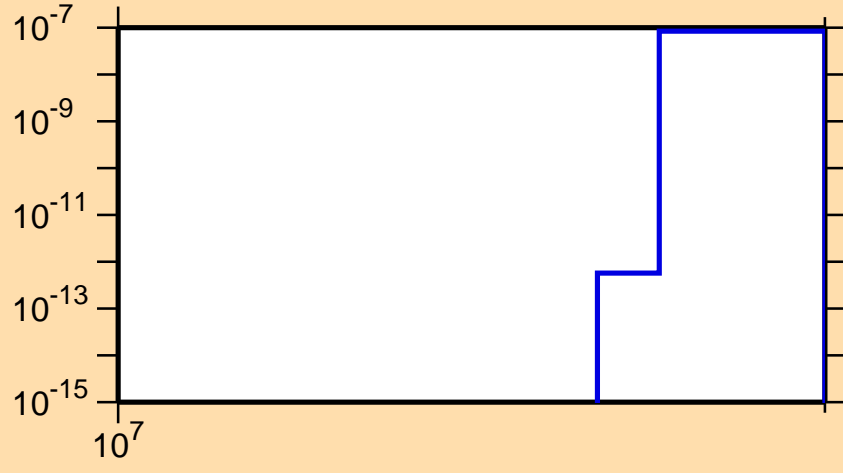
\sigma vs. E for ^{133}\text{Cs}(n,2np)
