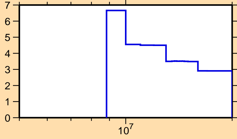
\Delta\sigma/\sigma vs. E for ^{133}\text{Cs}(n,2n)
