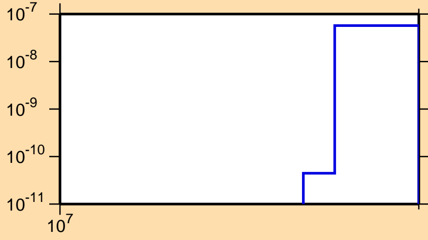
\sigma vs. E for ^{133}\text{Cs}(n,nt)
