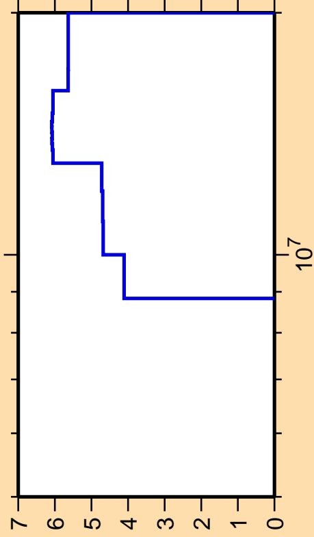
\Delta\sigma/\sigma vs. E for ^{133}\text{Cs}(n,n\text{cont.})
