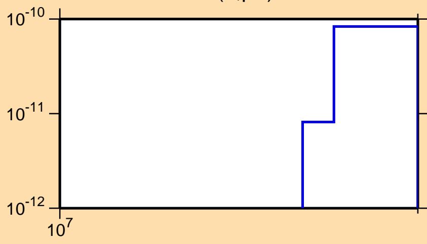
\sigma vs. E for ^{133}\text{Cs}(n,p\alpha)
