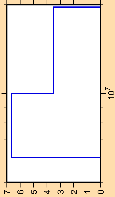
\Delta\sigma/\sigma vs. E for ^{133}\text{Cs}(n,2n)
