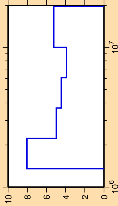
\Delta\sigma/\sigma vs. E for ^{133}\text{Cs}(n, ncont.)
