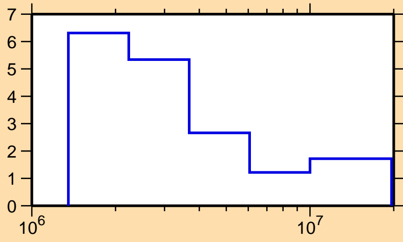
\Delta\sigma/\sigma vs. E for ^{133}\text{Cs}(n, tot.)
