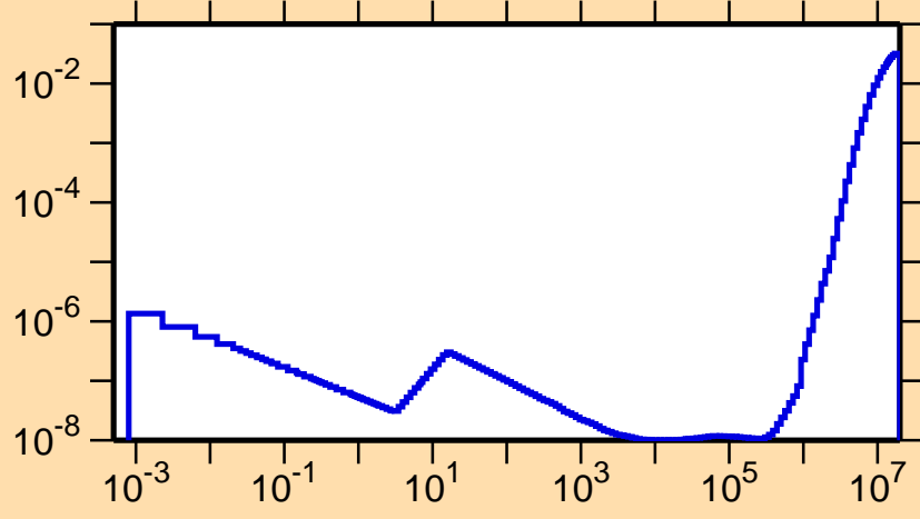
\sigma vs. E for ^{134}\text{Cs}(n,p)
