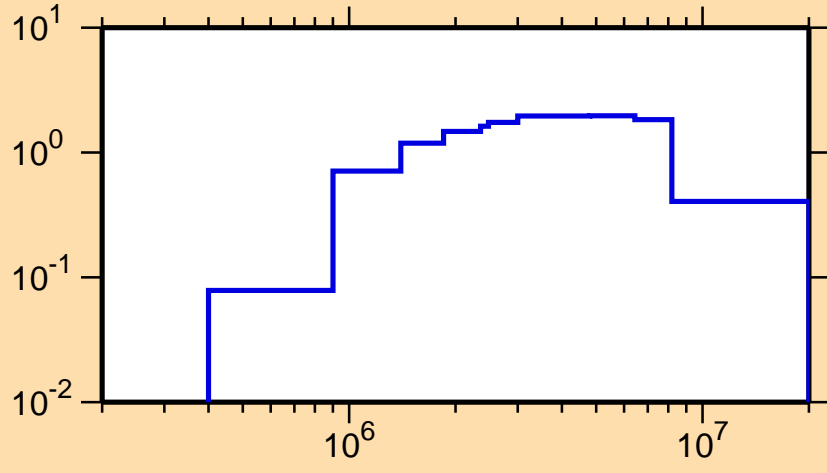
\sigma vs. E for ^{134}\text{Cs}(n,n\text{cont.})
