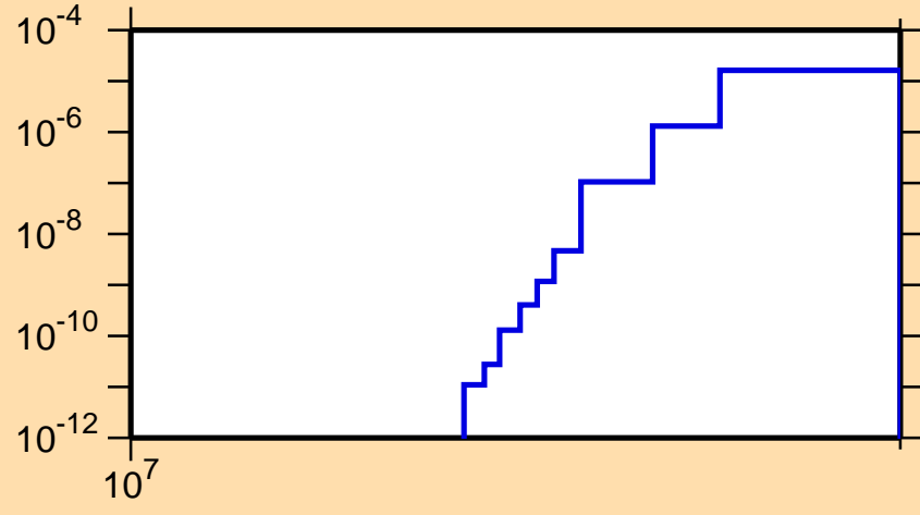
\sigma vs. E for ^{134}\text{Cs}(n,nd)
