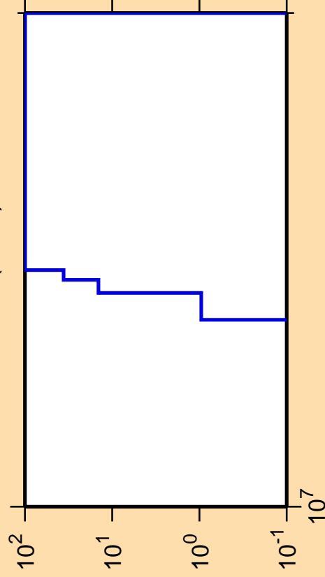
\Delta\sigma/\sigma vs. E for ^{134}\text{Cs}(n,nd)
