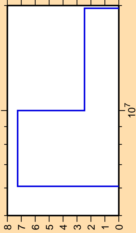
\Delta\sigma/\sigma vs. E for ^{134}\text{Cs}(n,2n)
