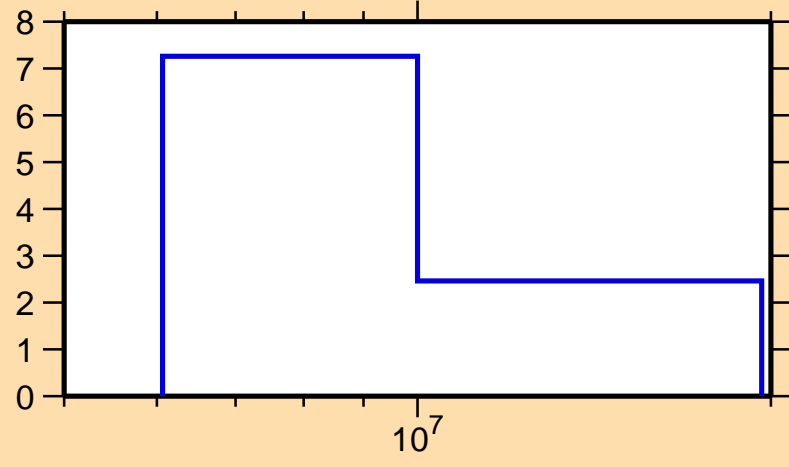
\Delta\sigma/\sigma vs. E for ^{134}\text{Cs}(n,2n)
