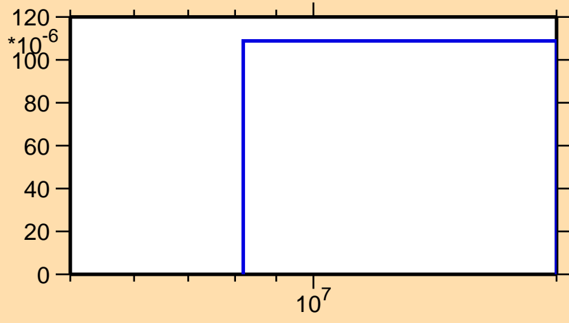
\sigma vs. E for ^{134}\text{Cs}(n,t)
