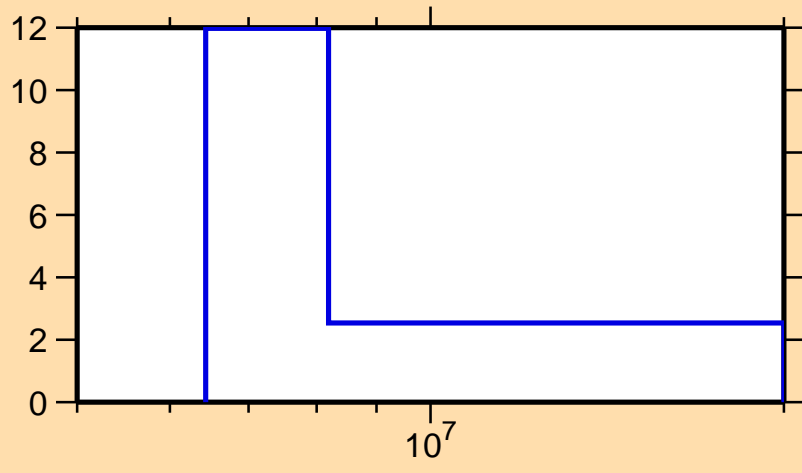
\Delta\sigma/\sigma vs. E for ^{134}\text{Cs}(n,2n)
