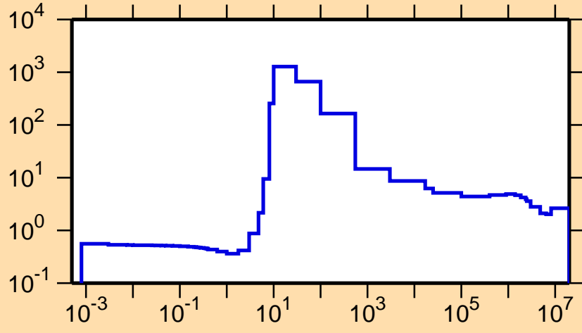
\sigma vs. E for ^{134}\text{Cs}(n,\text{el.})
