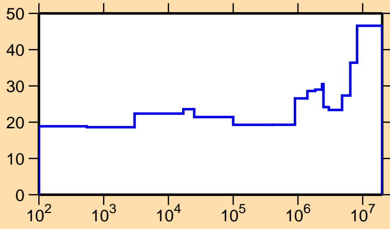
\Delta\sigma/\sigma vs. E for ^{134}\text{Cs}(n,n_1)
