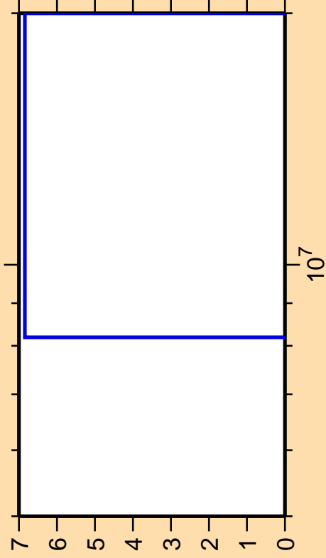
\Delta\sigma/\sigma vs. E for ^{134}\text{Cs}(n,3n)
