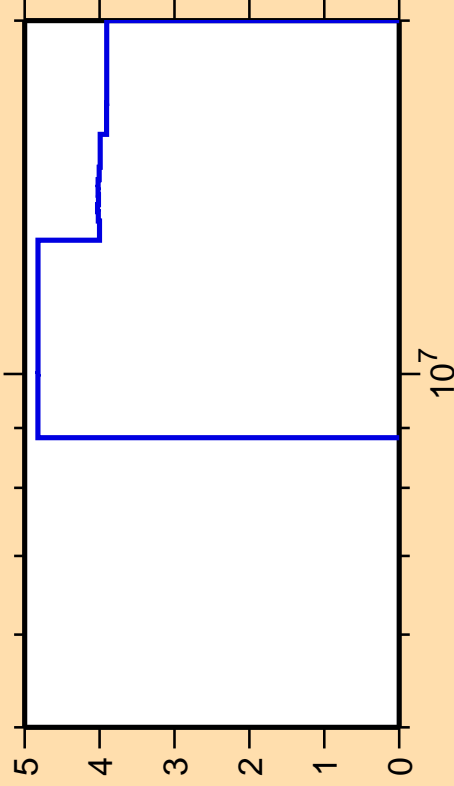
\Delta\sigma/\sigma vs. E for ^{135}\text{Cs}(n,2n)
