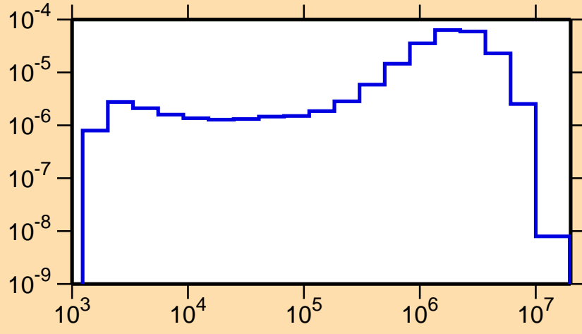
\sigma vs. E for ^{135}\text{Cs}(n,n_3)
