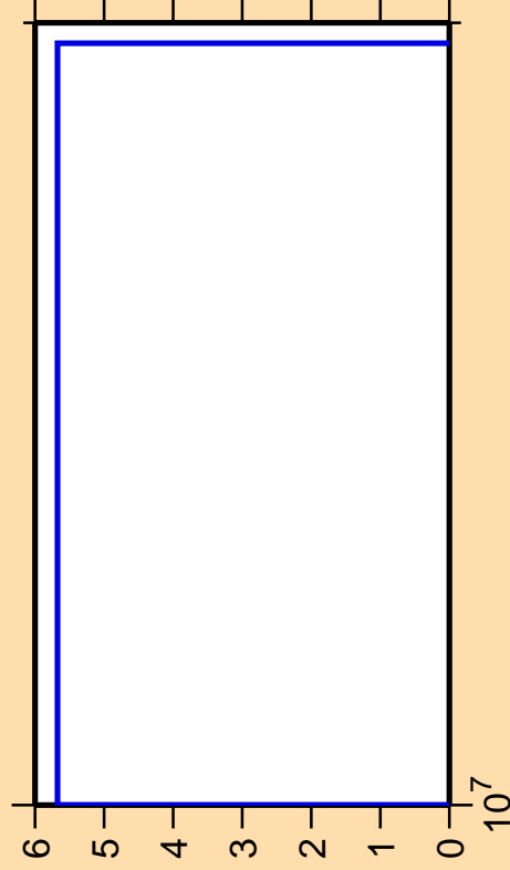
\Delta\sigma/\sigma vs. E for ^{136}\text{Cs}(n,\text{He3})
