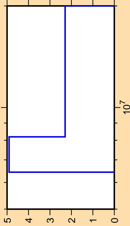
\Delta\sigma/\sigma vs. E for ^{136}\text{Cs}(n,2n)
