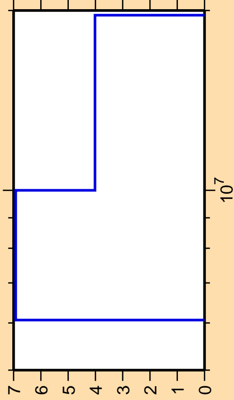
\Delta\sigma/\sigma vs. E for ^{136}\text{Cs}(n,2n)
