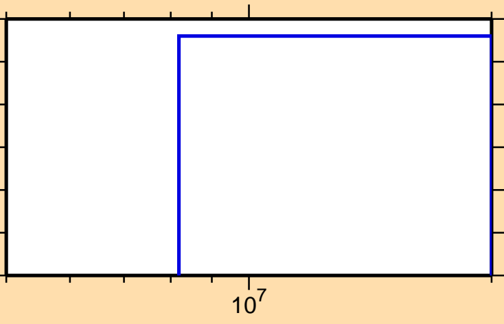
\sigma vs. E for ^{136}\text{Cs}(n,2np)
