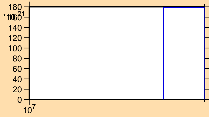
\sigma vs. E for ^{137}\text{Cs} (mt 11)
