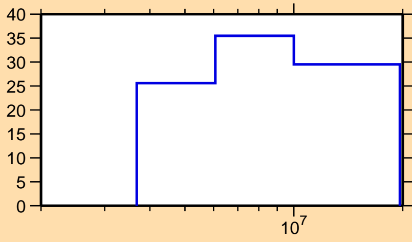
\Delta\sigma/\sigma vs. E for ^{137}\text{Cs}(n,p)
