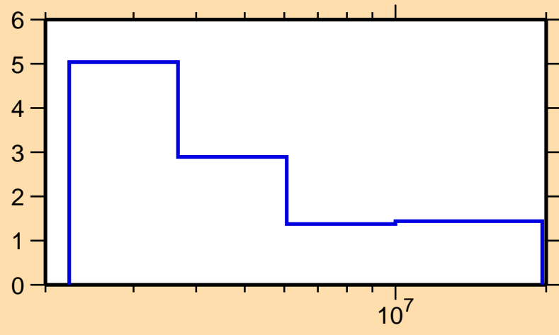
\Delta\sigma/\sigma vs. E for ^{137}\text{Cs}(n, tot.)
