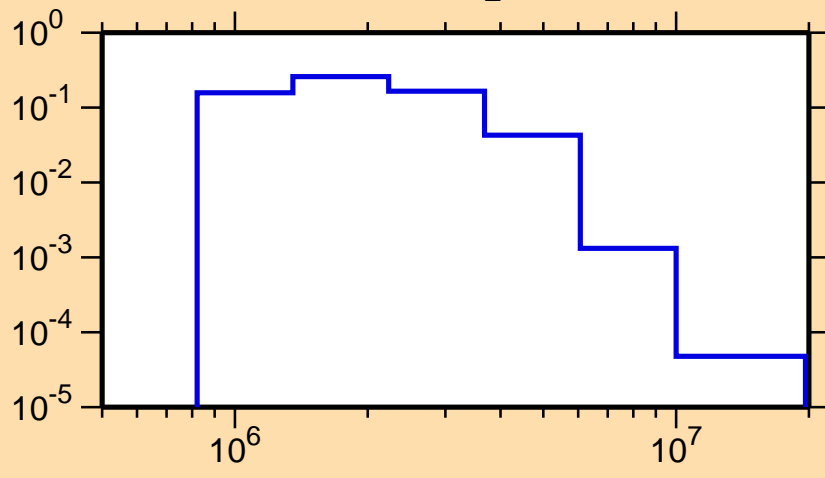
\sigma vs. E for ^{137}\text{Cs}(n,n_2)
