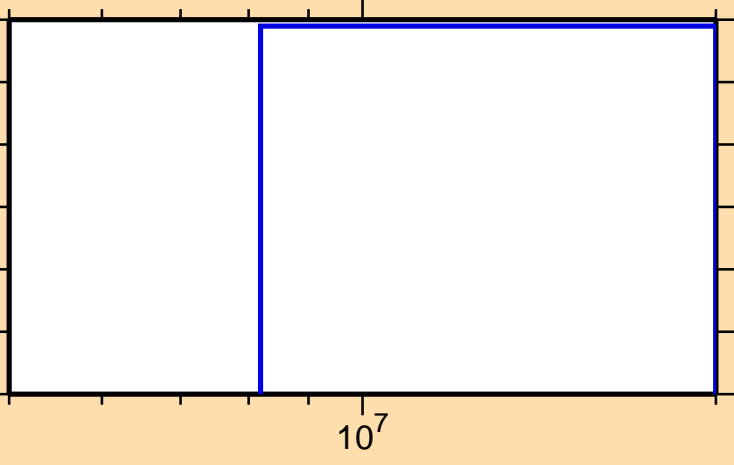
\sigma vs. E for ^{137}\text{Cs}(n,np)
