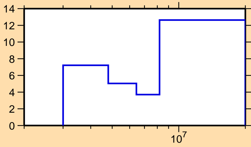
\Delta\sigma/\sigma vs. E for ^{137}\text{Cs}(n,n\text{cont.})
