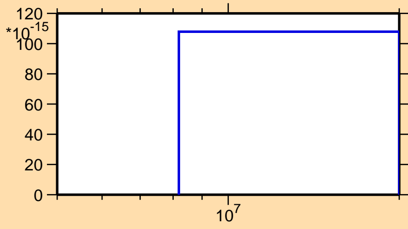
\sigma vs. E for ^{137}\text{Cs}(n,2n\alpha)
