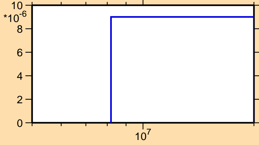
\sigma vs. E for ^{137}\text{Cs}(n,n\alpha)
