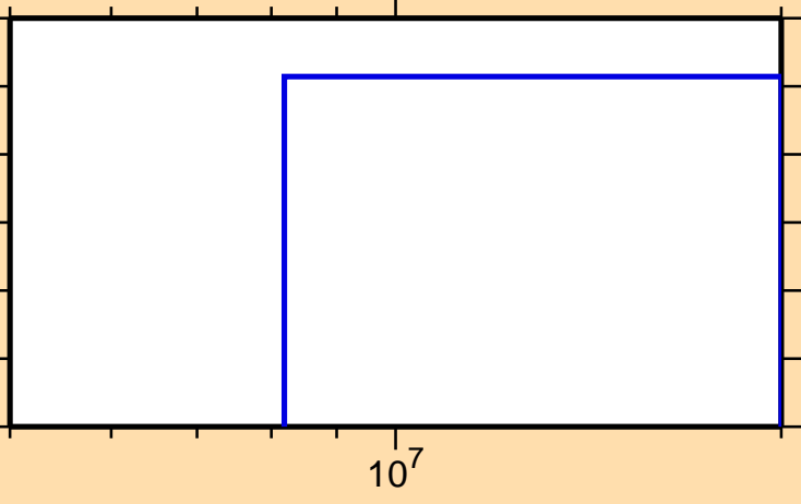
\sigma vs. E for ^{137}\text{Cs}(n,p\alpha)
