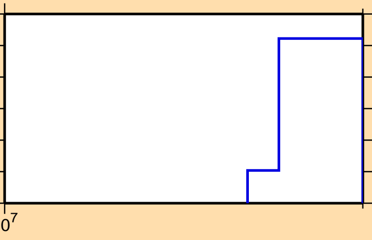
\sigma vs. E for ^{138}\text{Cs}(n,p\alpha)
