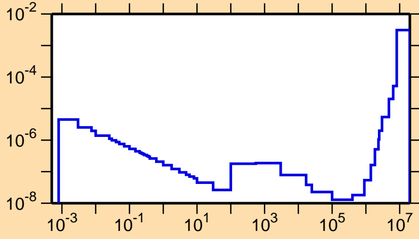
\sigma vs. E for ^{138}\text{Cs}(n,\alpha)
