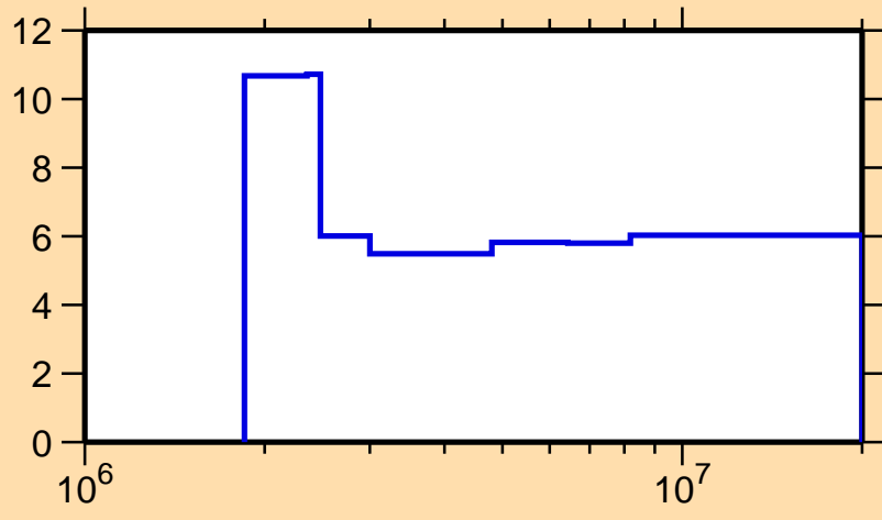
\Delta\sigma/\sigma vs. E for ^{138}\text{Cs}(n,\text{nonel.})
