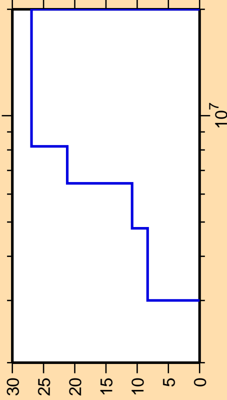
\Delta\sigma/\sigma vs. E for ^{138}\text{Cs}(n,n\text{cont.})
