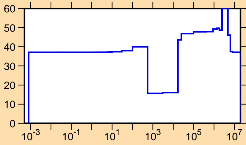
\Delta\sigma/\sigma vs. E for ^{138}\text{Cs}(n,\gamma)
