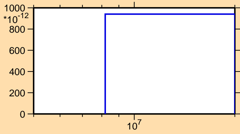
\sigma vs. E for ^{138}\text{Cs}(n,2n\alpha)
