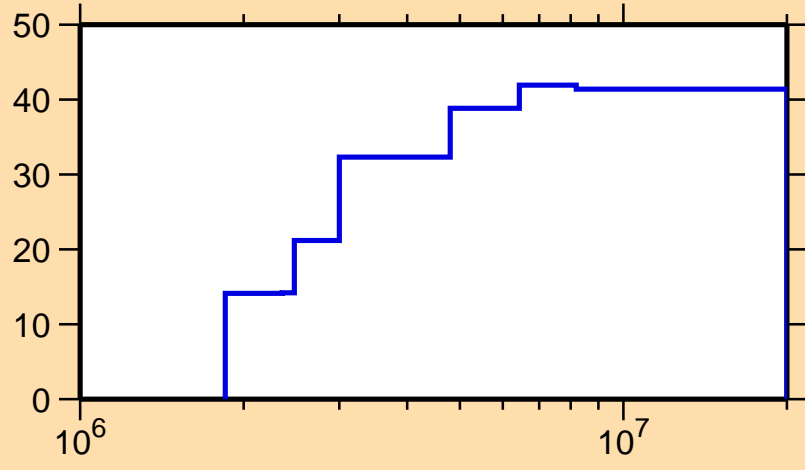
\Delta\sigma/\sigma vs. E for ^{138}\text{Cs}(n, n_1)
