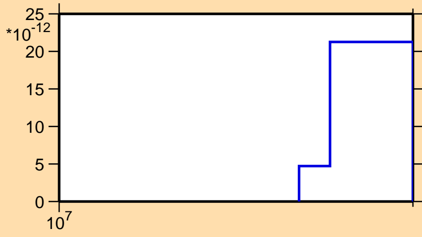
\sigma vs. E for ^{138}\text{Cs}(n,p\alpha)
