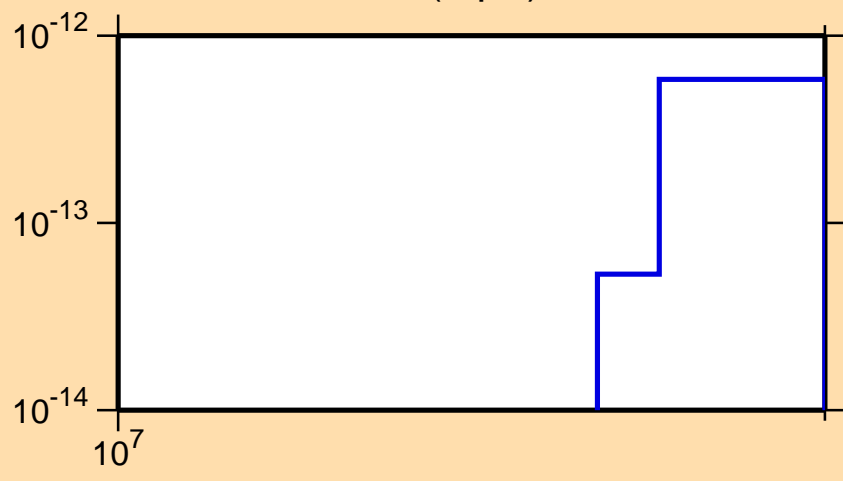
\sigma vs. E for ^{139}\text{Cs}(n,p\alpha)
