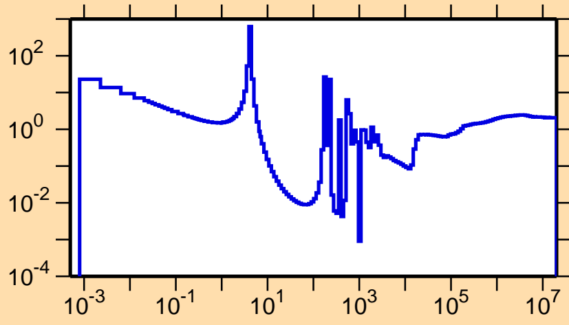
\sigma vs. E for ^{140}\text{Cs}(n,\text{nonel.})
