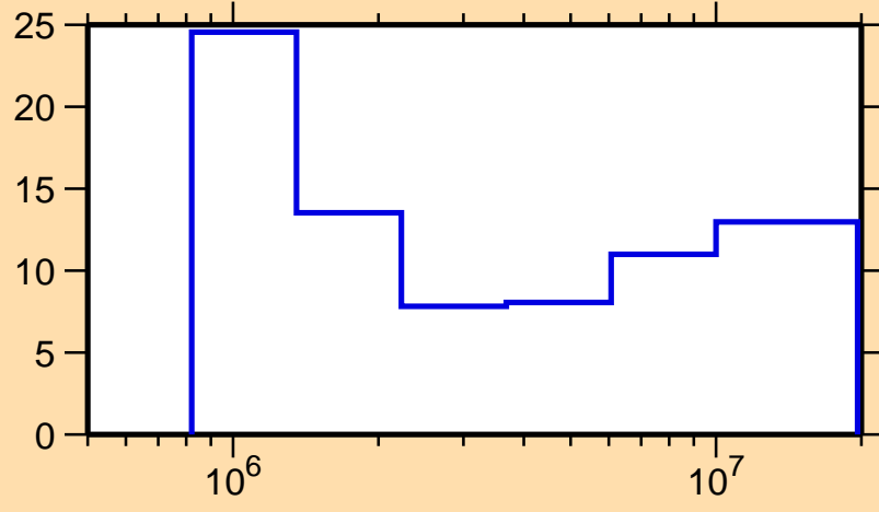
\Delta\sigma/\sigma vs. E for ^{140}\text{Cs}(n,\text{inel.})
