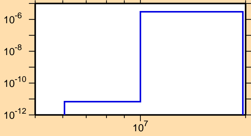
\sigma vs. E for ^{140}\text{Cs}(n,2n\alpha)
