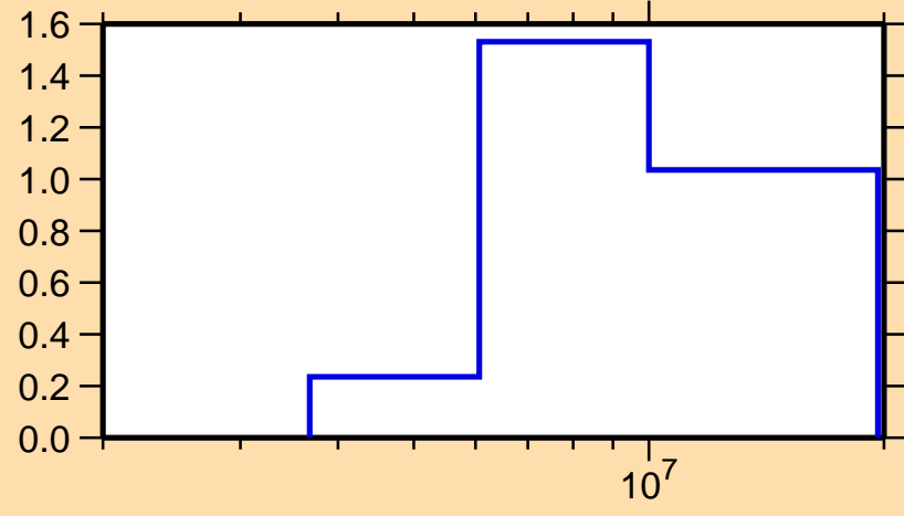
\sigma vs. E for ^{140}\text{Cs}(n,2n)
