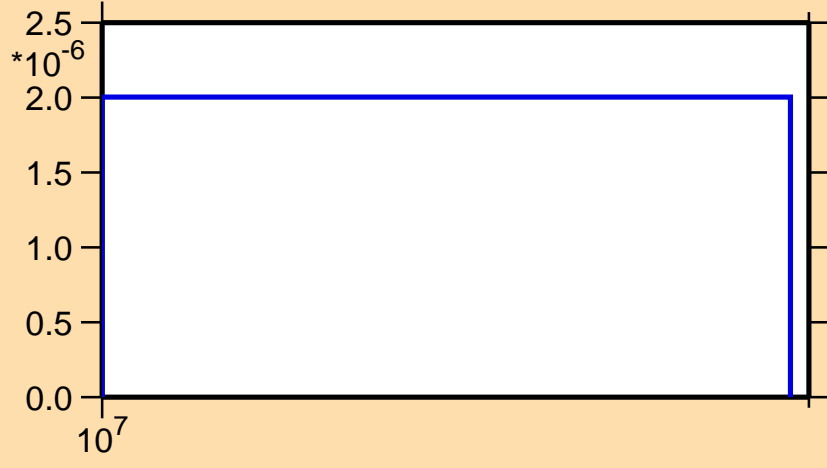
\sigma vs. E for ^{140}\text{Cs}(n,\text{nd})
