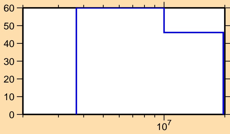
\Delta\sigma/\sigma vs. E for ^{140}\text{Cs}(n,p)
