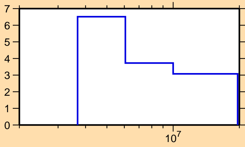
\Delta\sigma/\sigma vs. E for ^{140}\text{Cs}(n,\text{tot.})
