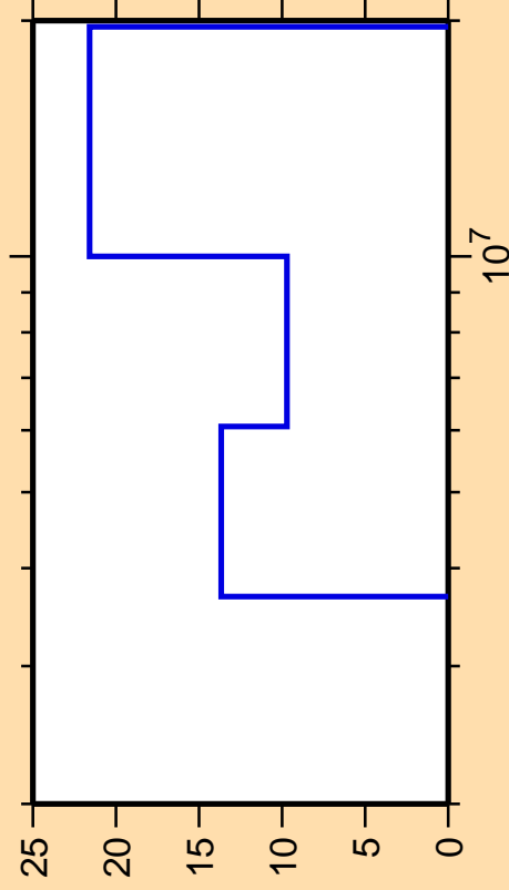
\Delta\sigma/\sigma vs. E for ^{140}\text{Cs}(n,2n)
