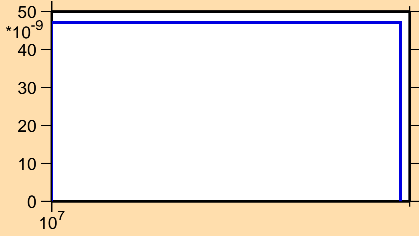
\sigma vs. E for ^{140}\text{Cs}(n,2np)
