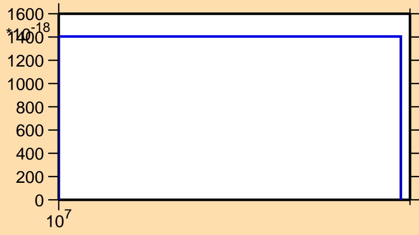
\sigma vs. E for ^{140}\text{Cs}(n,p\alpha)
