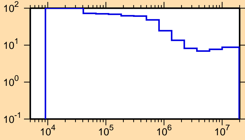
\Delta\sigma/\sigma vs. E for ^{140}\text{Cs}(n,\text{nonel.})
