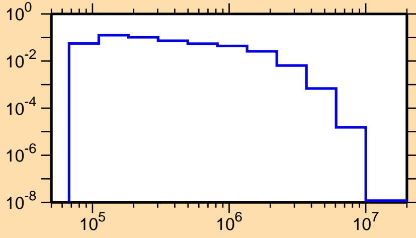
\sigma vs. E for ^{140}\text{Cs}(n,n_3)
