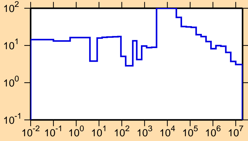
\Delta\sigma/\sigma vs. E for ^{140}\text{Cs}(n,\text{tot.})
