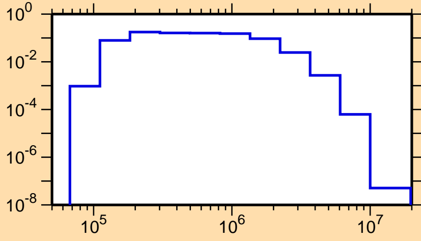
\sigma vs. E for ^{140}\text{Cs}(n,n_4)
