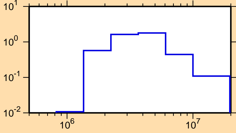
\sigma vs. E for ^{140}\text{Cs}(n,n\text{cont.})
