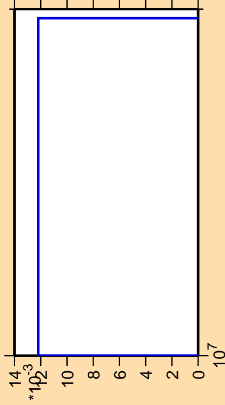
\Delta\sigma/\sigma vs. E for ^{140}\text{Cs}(n,p\alpha)
