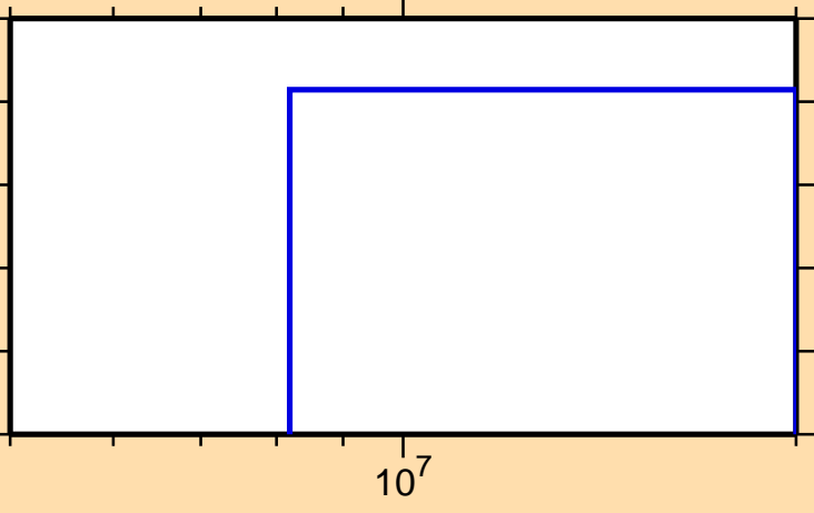
\sigma vs. E for ^{140}\text{Cs}(n,2np)
