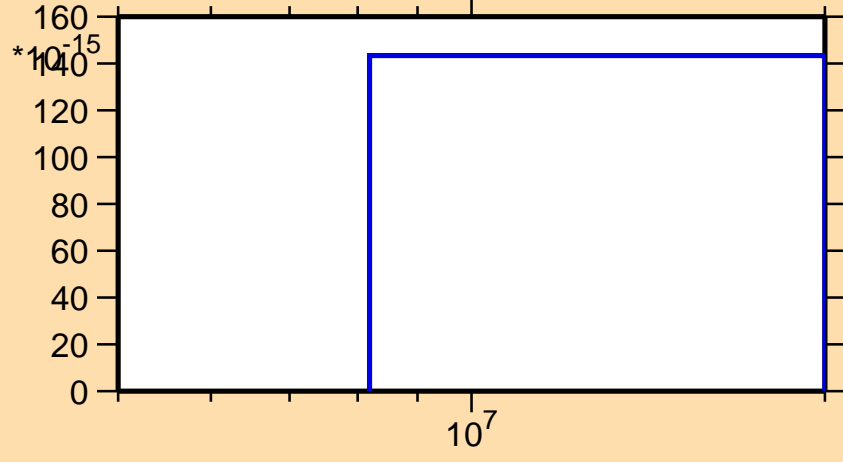
\sigma vs. E for ^{140}\text{Cs}(\text{mt } 11)
