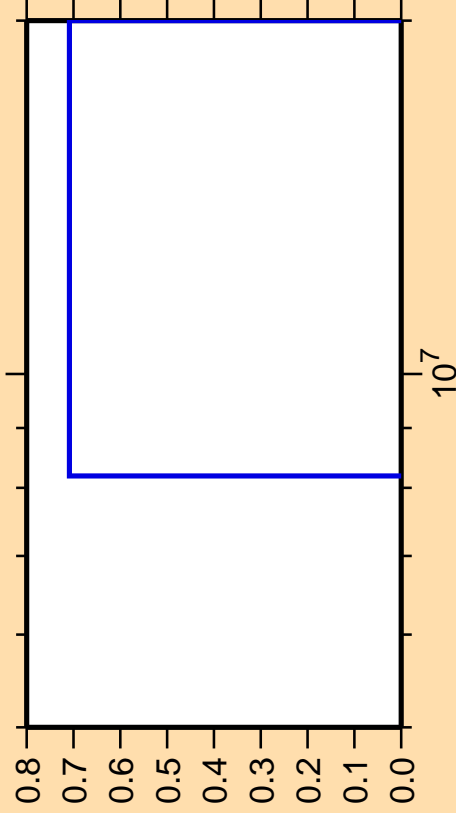
\Delta\sigma/\sigma vs. E for ^{140}\text{Cs}(\text{mt } 11)
