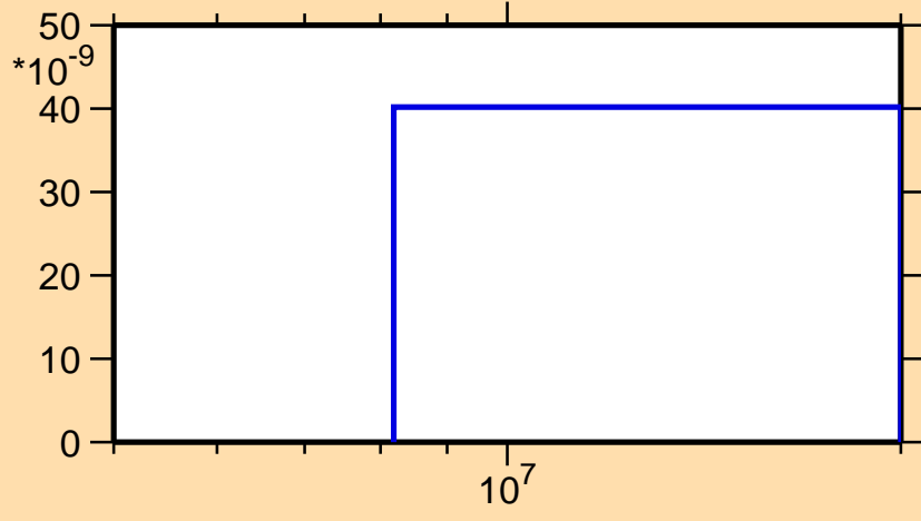
\sigma vs. E for ^{141}\text{Cs}(n,2n\alpha)
