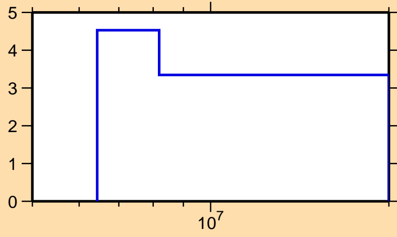
\Delta\sigma/\sigma vs. E for ^{141}\text{Cs}(n,\text{tot.})
