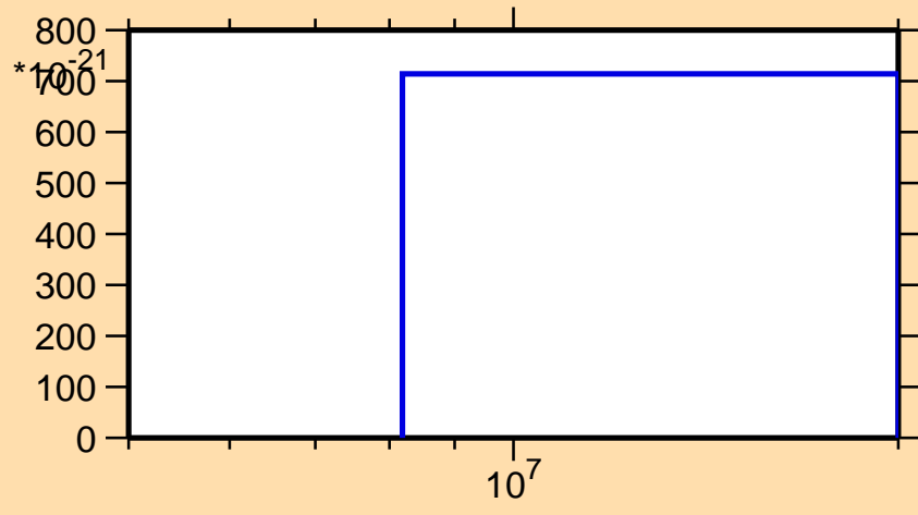
\sigma vs. E for ^{141}\text{Cs} (mt 42)
