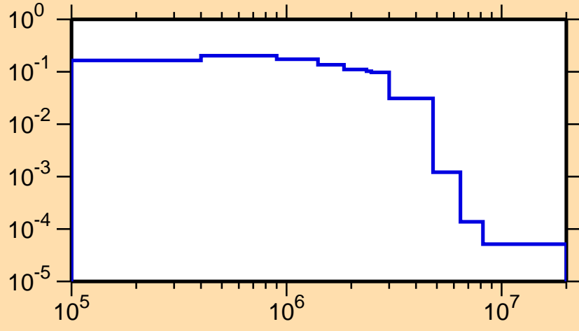
\sigma vs. E for ^{141}\text{Cs}(n,n_2)
