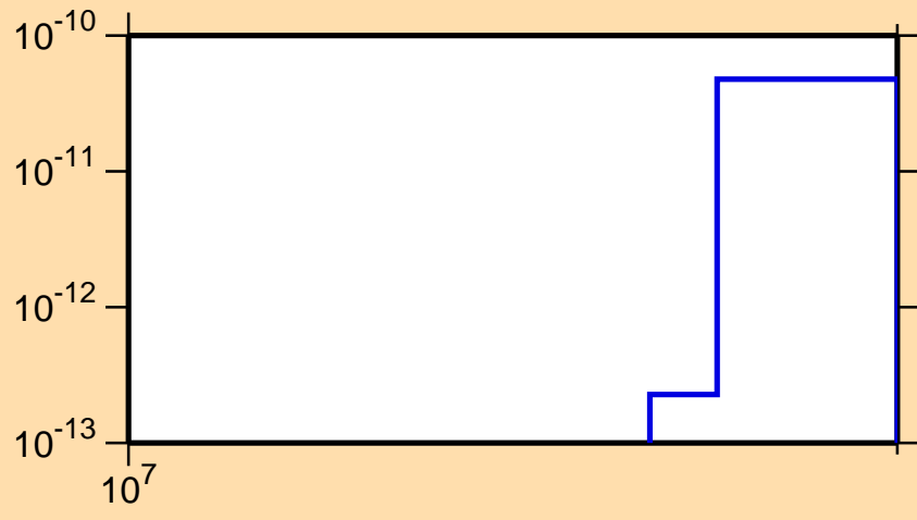
\sigma vs. E for ^{142}\text{Cs}(n,3n\alpha)
