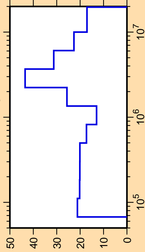
\Delta\sigma/\sigma vs. E for ^{142}\text{Cs}(n,n_3)
