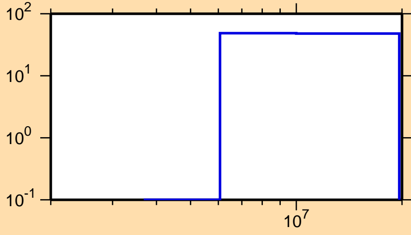
\Delta\sigma/\sigma vs. E for ^{142}\text{Cs}(n,p)
