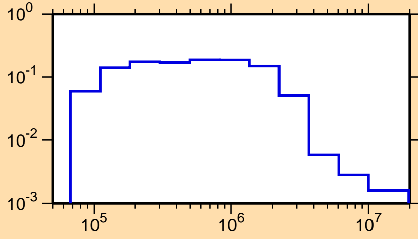
\sigma vs. E for ^{142}\text{Cs}(n,n_3)
