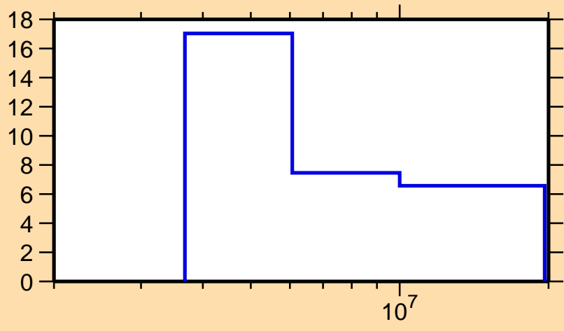
\Delta\sigma/\sigma vs. E for ^{142}\text{Cs}(n,\text{el.})
