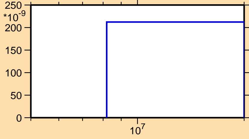
\sigma vs. E for ^{142}\text{Cs}(n,2n\alpha)
