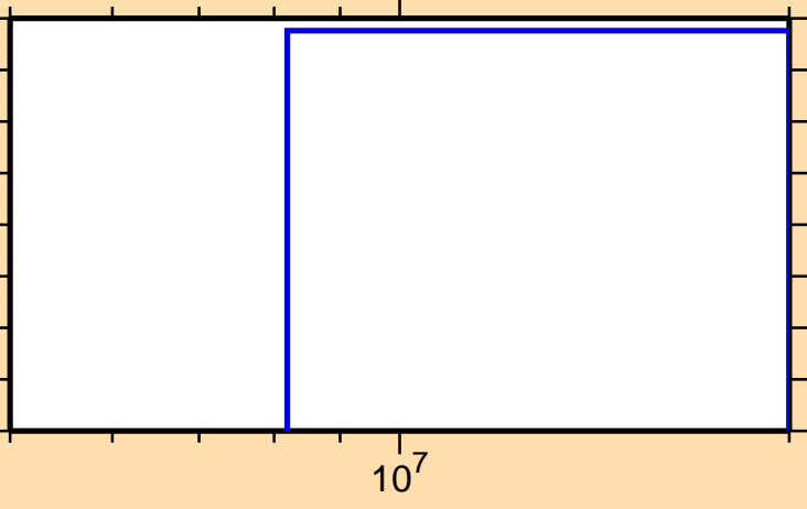
\sigma vs. E for ^{142}\text{Cs}(n,\text{nd})
