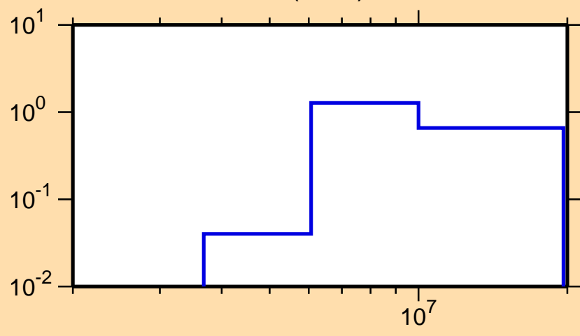
\sigma vs. E for ^{143}\text{Cs}(n,2n)
