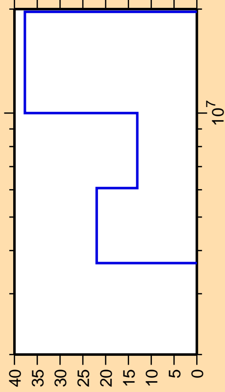
\Delta\sigma/\sigma vs. E for ^{143}\text{Cs}(n,2n)
