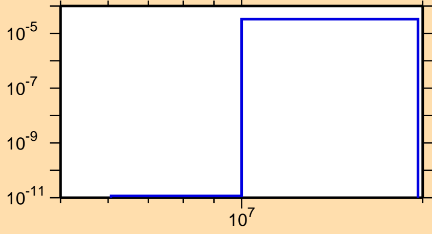
\sigma vs. E for ^{143}\text{Cs}(n,n\alpha)
