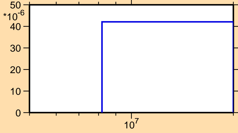
\sigma vs. E for ^{143}\text{Cs}(n,d)
