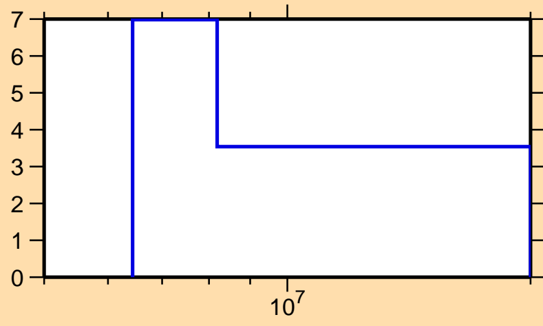
\Delta\sigma/\sigma vs. E for ^{143}\text{Cs}(n,\text{tot.})
