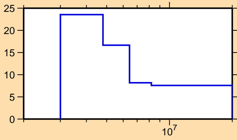
\Delta\sigma/\sigma vs. E for ^{143}\text{Cs}(n, el.)
