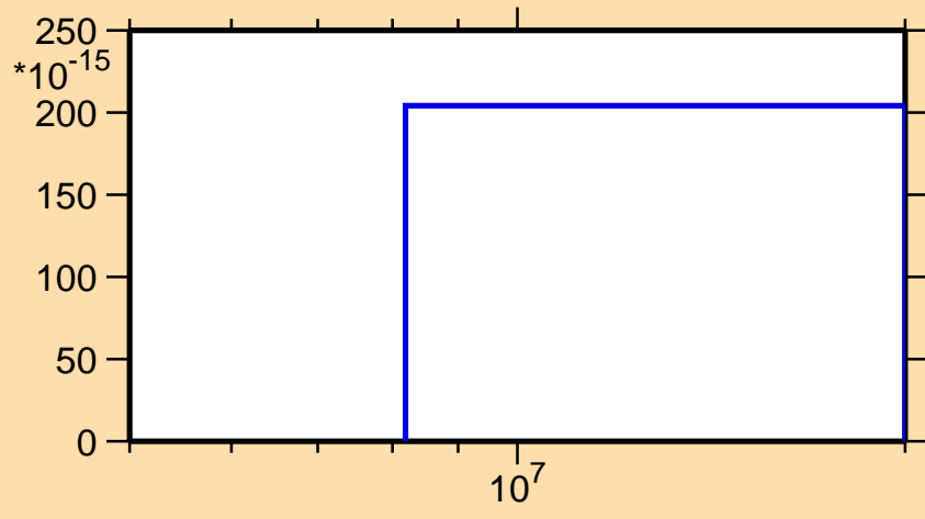
\sigma vs. E for ^{143}\text{Cs}(n,3n\alpha)
