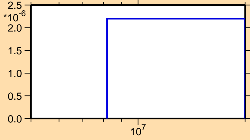
\sigma vs. E for ^{143}\text{Cs}(n,nt)
