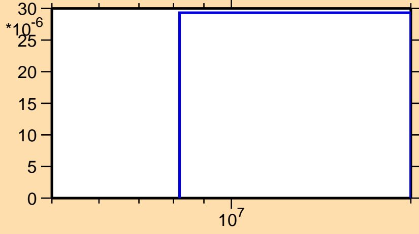
\sigma vs. E for ^{143}\text{Cs}(n,t)
