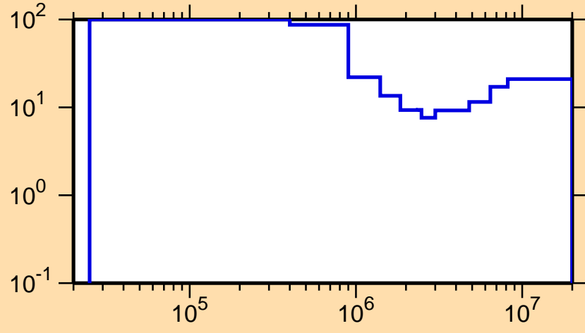
\Delta\sigma/\sigma vs. E for ^{143}\text{Cs}(n,\text{inel.})
