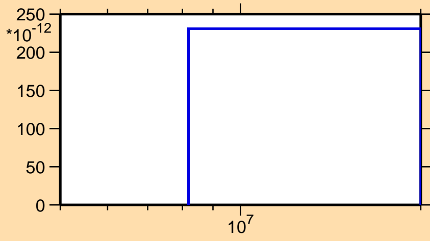
\sigma vs. E for ^{143}\text{Cs}(n,2np)
