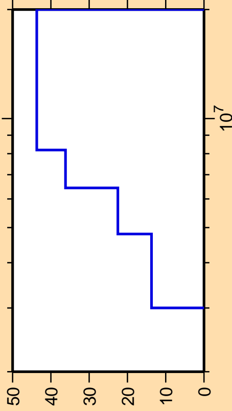
\Delta\sigma/\sigma vs. E for ^{143}\text{Cs}(n, ncont.)
