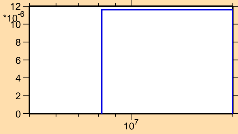
\sigma vs. E for ^{143}\text{Cs}(n,np)
