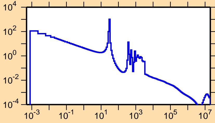
\sigma vs. E for ^{144}\text{Cs}(n,\gamma)
