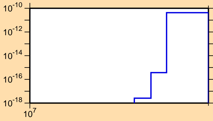
\sigma vs. E for ^{144}\text{Cs} (mt 11)
