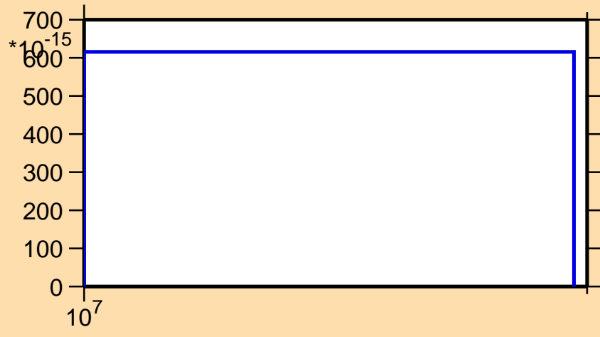
\sigma vs. E for ^{144}\text{Cs}(n,3n\alpha)
