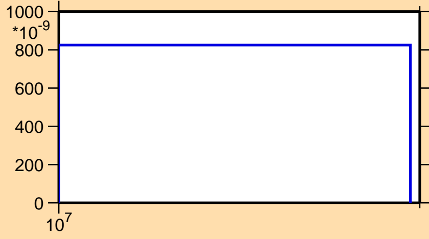
\sigma vs. E for ^{144}\text{Cs}(n,\text{nd})
