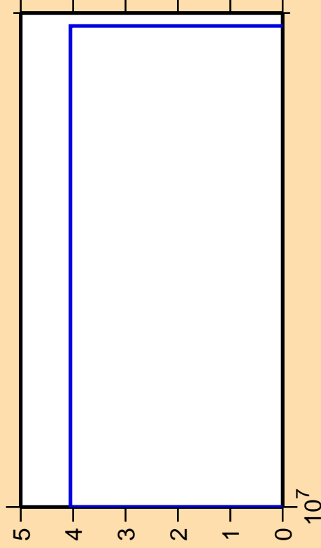
\Delta\sigma/\sigma vs. E for ^{144}\text{Cs}(n,3n\alpha)
