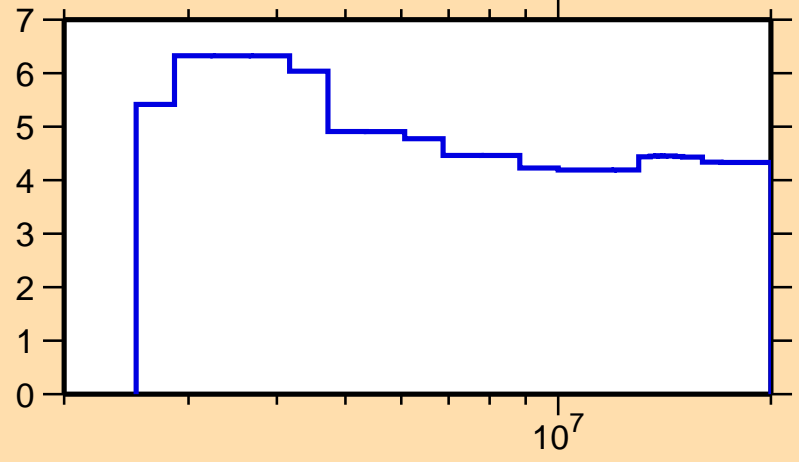
\Delta\sigma/\sigma vs. E for ^{58}\text{Cu}(n,n\text{onel.})
