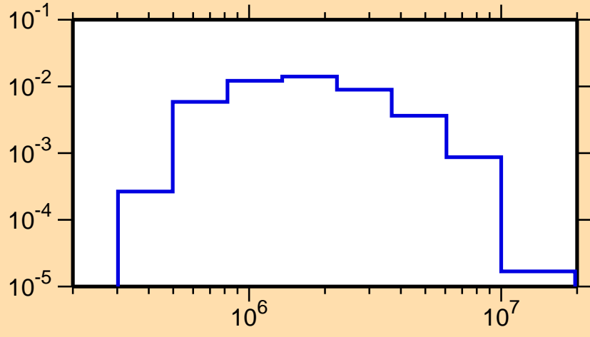
\sigma vs. E for ^{58}\text{Cu}(n,n_2)
