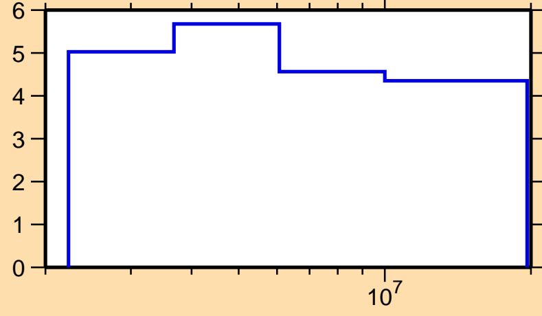
\Delta\sigma/\sigma vs. E for ^{58}\text{Cu}(n,n\text{nonel.})
