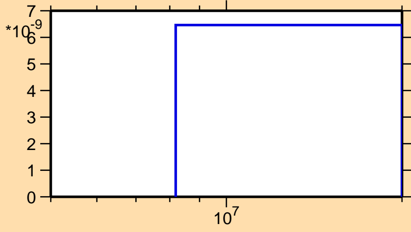
\sigma vs. E for ^{58}\text{Cu} (mt 45)
