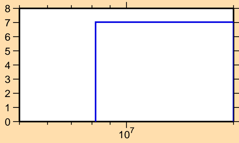
\Delta\sigma/\sigma vs. E for ^{58}\text{Cu}(n,\text{el.})
