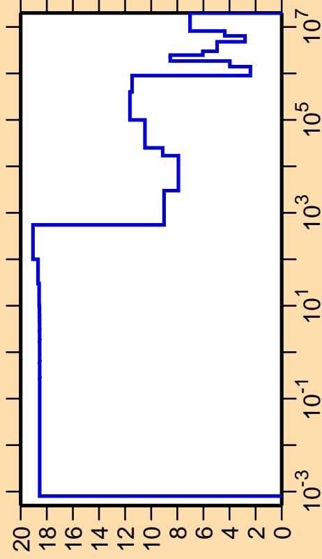
\Delta\sigma/\sigma vs. E for ^{58}\text{Cu}(n,\text{el.})
