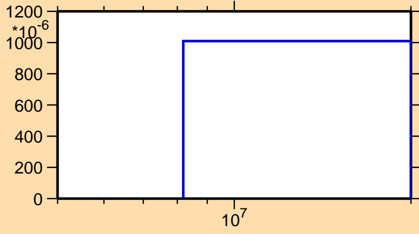
\sigma vs. E for ^{58}\text{Cu}(n,\text{pd})
