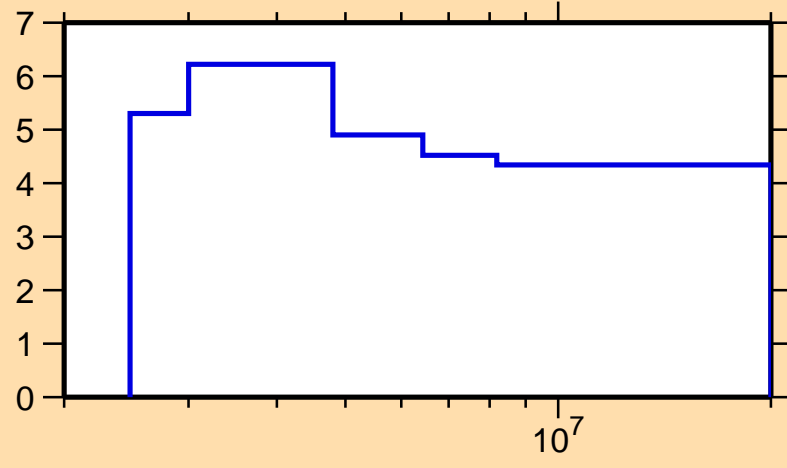
\Delta\sigma/\sigma vs. E for ^{58}\text{Cu}(n,n\text{onel.})
