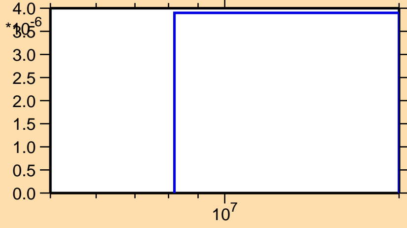
\sigma vs. E for ^{58}\text{Cu}(n,2np)
