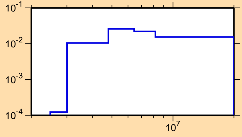
\sigma vs. E for ^{58}\text{Cu}(n,n\text{cont.})
