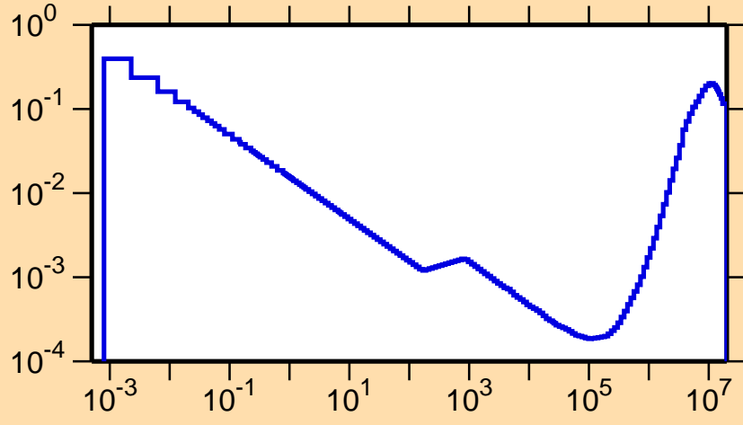
\sigma vs. E for ^{59}\text{Cu}(n,\alpha)
