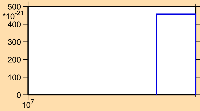
\sigma vs. E for ^{59}\text{Cu}(n,2n\alpha)
