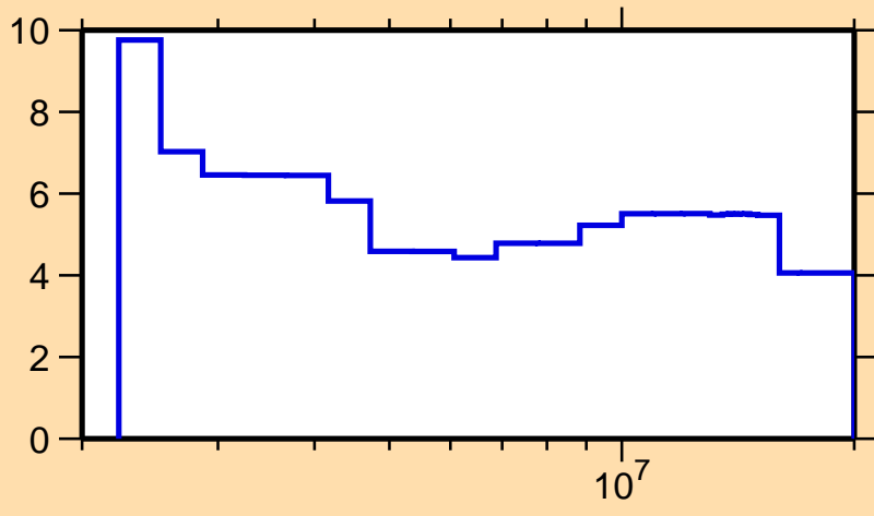
\Delta\sigma/\sigma vs. E for ^{59}\text{Cu}(n, el.)
