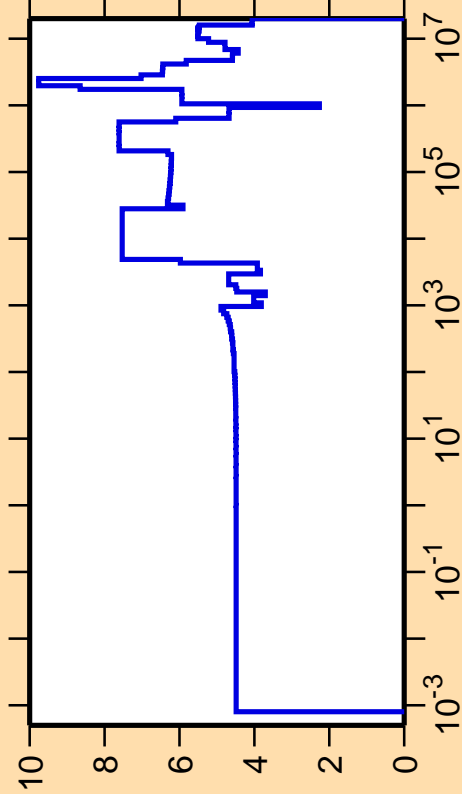
\Delta\sigma/\sigma vs. E for ^{59}\text{Cu}(n,\text{el.})
