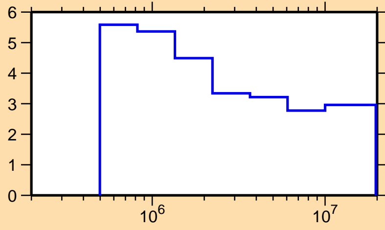
\Delta\sigma/\sigma vs. E for ^{59}\text{Cu}(n,\text{nonel.})
