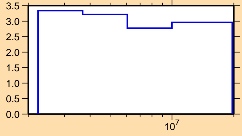
\Delta\sigma/\sigma vs. E for ^{59}\text{Cu}(n,n\text{nonel.})
