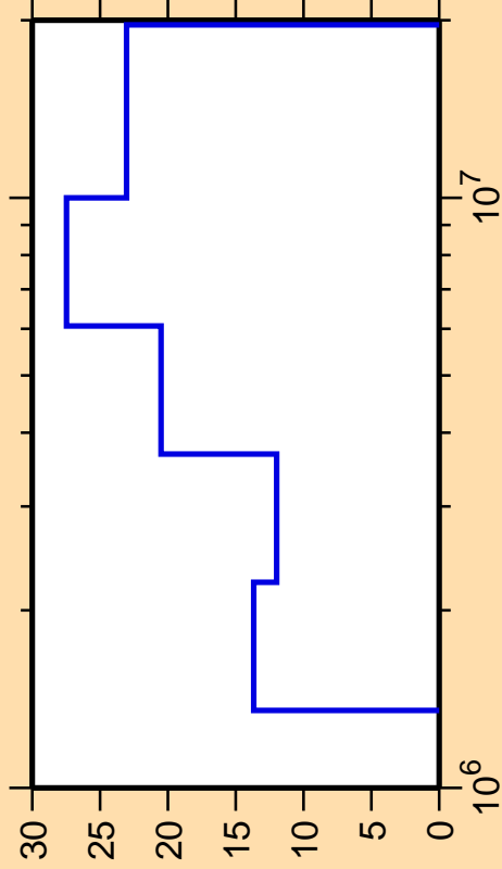
\Delta\sigma/\sigma vs. E for ^{59}\text{Cu}(n,n_4)
