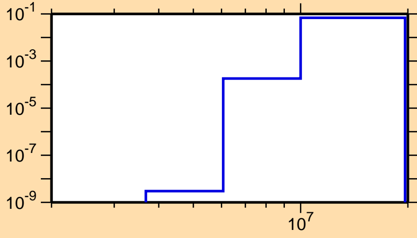
\sigma vs. E for ^{59}\text{Cu}(n,p\alpha)
