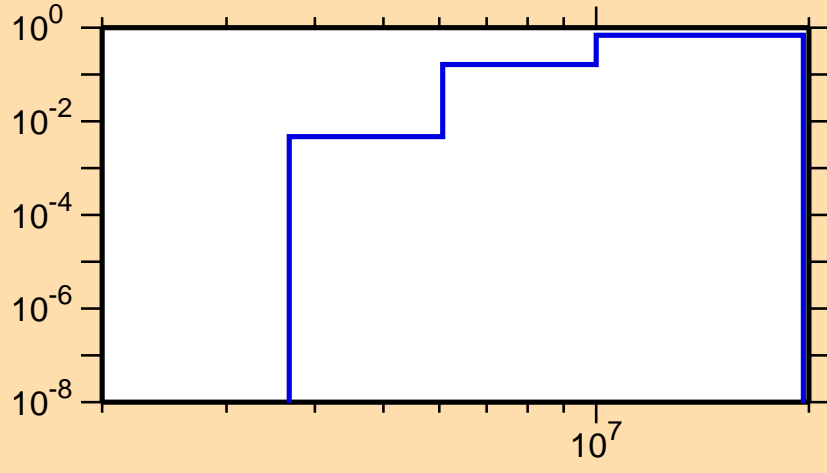
\sigma vs. E for ^{59}\text{Cu}(n,np)
