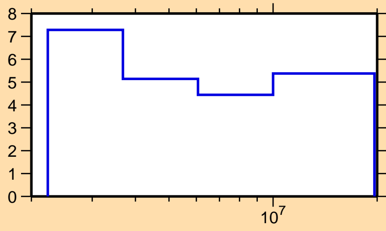
\Delta\sigma/\sigma vs. E for ^{59}\text{Cu}(n,\text{el.})
