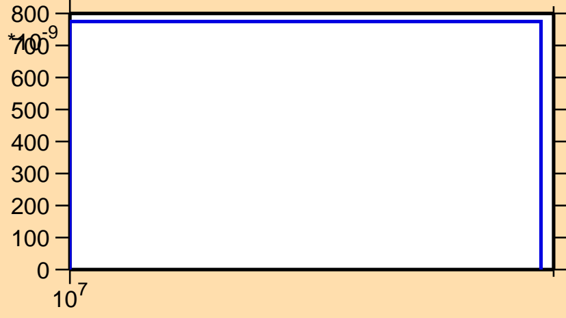
\sigma vs. E for ^{59}\text{Cu}(n,\text{nd})
