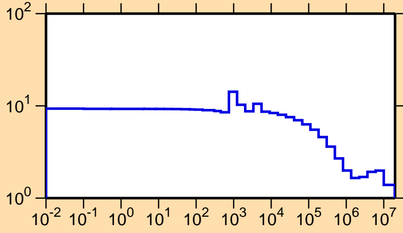
\sigma vs. E for ^{59}\text{Cu}(n,\text{el.})
