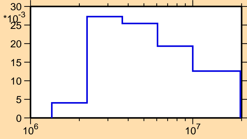
\sigma vs. E for ^{59}\text{Cu}(n,n_4)
