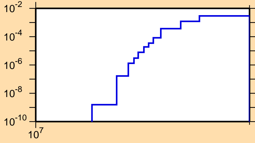
\sigma vs. E for ^{60}\text{Cu}(n,\text{nd})
