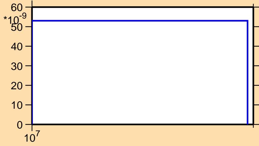
\sigma vs. E for ^{60}\text{Cu}(n,\text{pt})
