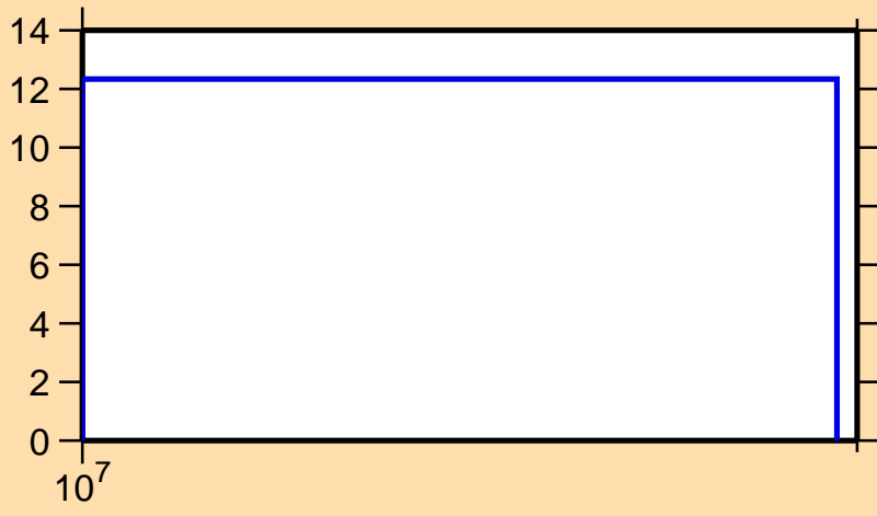
\Delta\sigma/\sigma vs. E for ^{60}\text{Cu}(n,\text{inel.})
