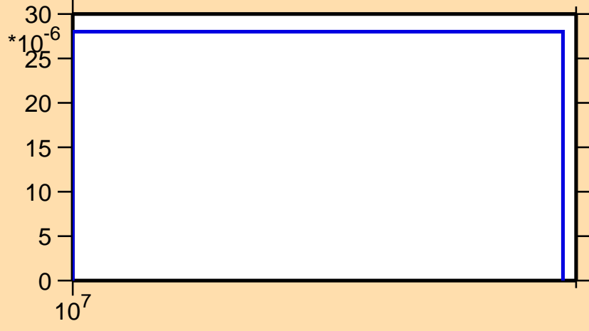
\sigma vs. E for ^{60}\text{Cu}(n,\text{pd})
