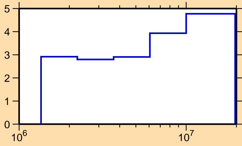
\Delta\sigma/\sigma vs. E for ^{60}\text{Cu}(n,\text{el.})
