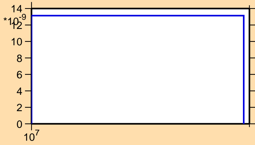
\sigma vs. E for ^{60}\text{Cu}(\text{mt117})
