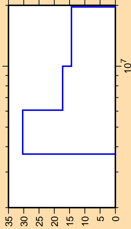
\Delta\sigma/\sigma vs. E for ^{60}\text{Cu}(n,np)
