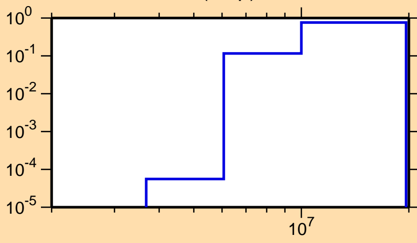
\sigma vs. E for ^{60}\text{Cu}(n,np)
