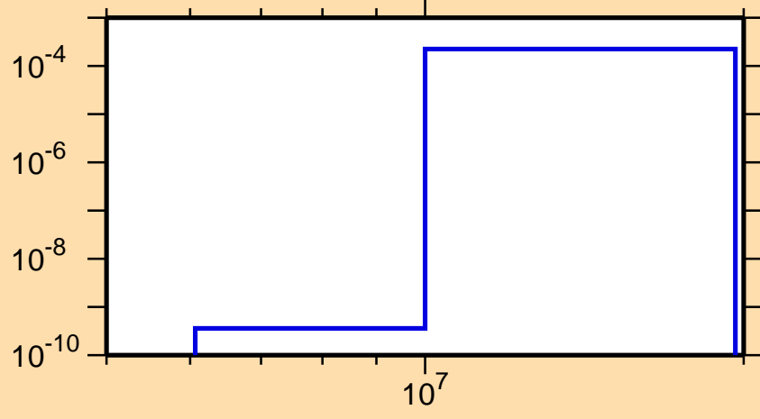
\sigma vs. E for ^{60}\text{Cu}(n,\text{He3})
