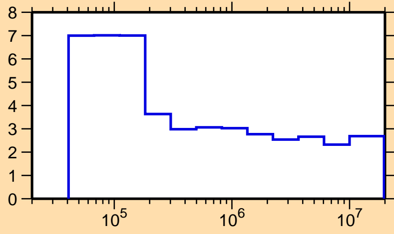
\Delta\sigma/\sigma vs. E for ^{60}\text{Cu}(n,\text{nonel.})
