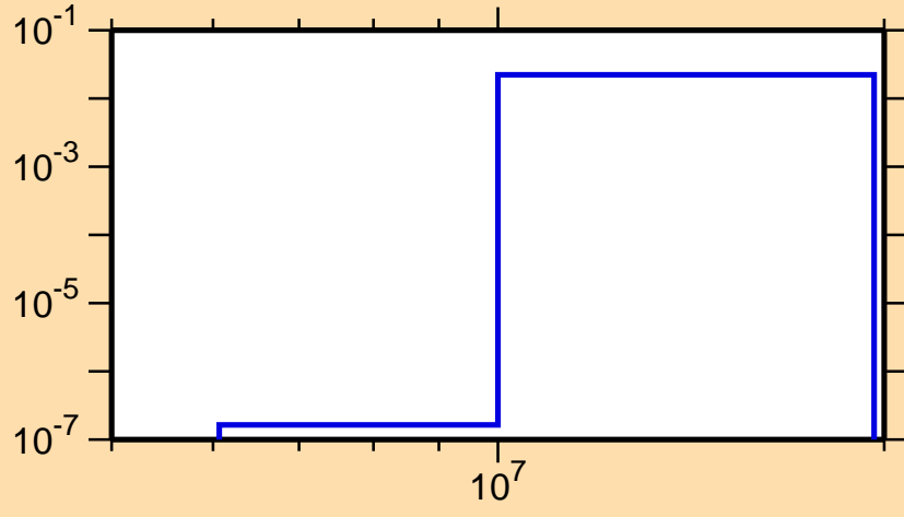
\sigma vs. E for ^{60}\text{Cu}(n,n\alpha)
