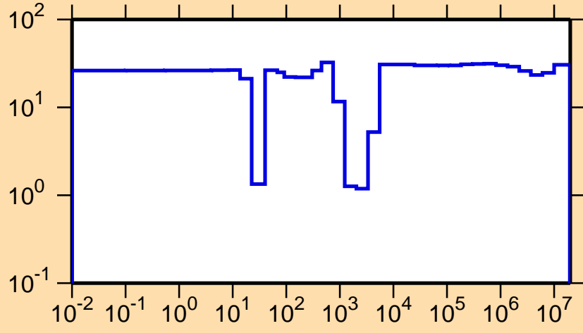
\Delta\sigma/\sigma vs. E for ^{60}\text{Cu}(n,\gamma)
