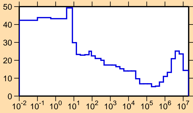
\Delta\sigma/\sigma vs. E for ^{60}\text{Cu}(n,p)
