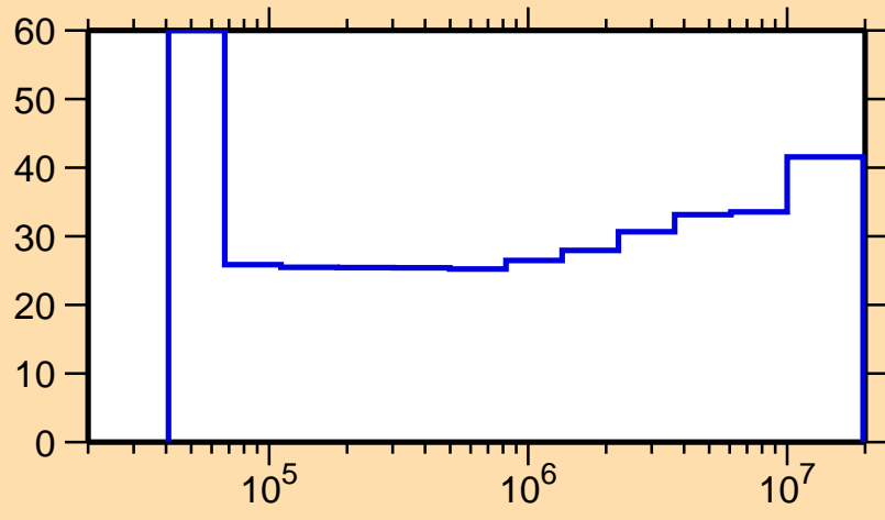
\Delta\sigma/\sigma vs. E for ^{60}\text{Cu}(n,n_1)
