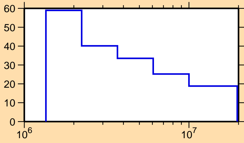
\Delta\sigma/\sigma vs. E for ^{60}\text{Cu}(n,n\text{cont.})
