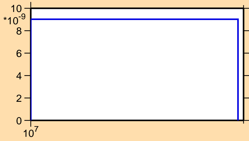
\sigma vs. E for ^{60}\text{Cu} (mt 45)
