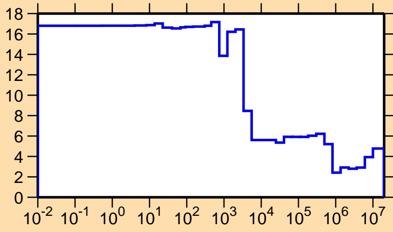
\Delta\sigma/\sigma vs. E for ^{60}\text{Cu}(n,\text{el.})
