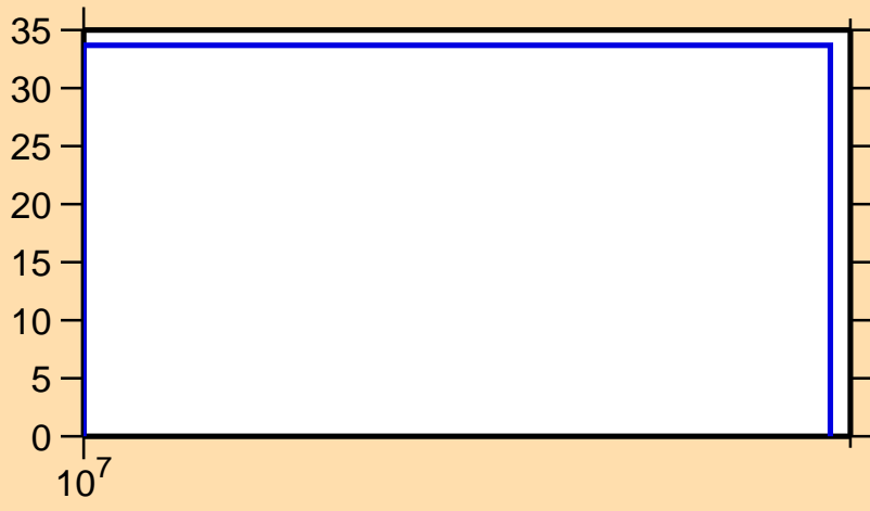
\Delta\sigma/\sigma vs. E for ^{60}\text{Cu}(n,2n)
