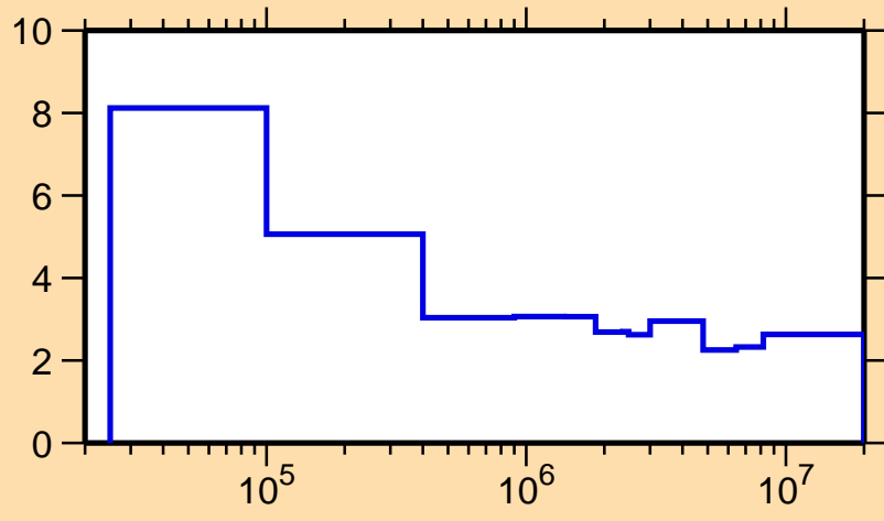
\Delta\sigma/\sigma vs. E for ^{60}\text{Cu}(n,\text{nonel.})
