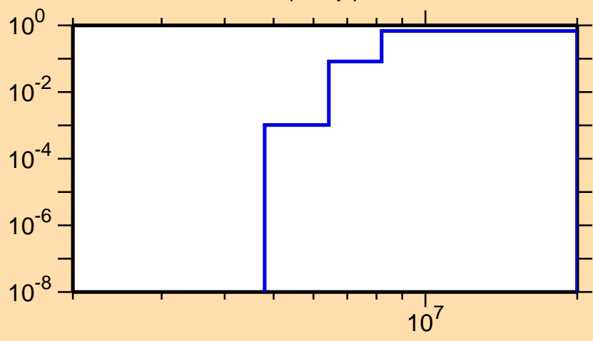
\sigma vs. E for ^{60}\text{Cu}(n,np)
