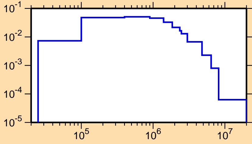
\sigma vs. E for ^{60}\text{Cu}(n,n_1)
