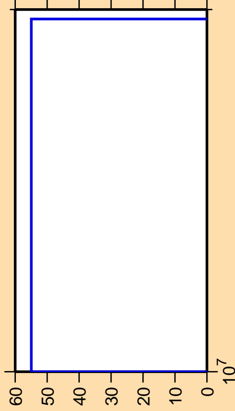
\Delta\sigma/\sigma vs. E for ^{61}\text{Cu}(n,nd)
