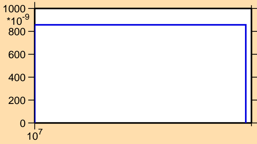
\sigma vs. E for ^{61}\text{Cu}(n,nd)
