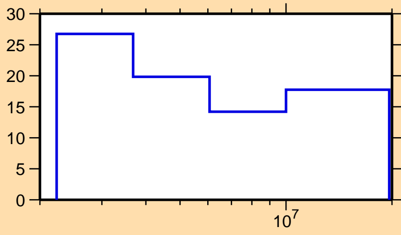
\Delta\sigma/\sigma vs. E for ^{61}\text{Cu}(n,n\text{cont.})
