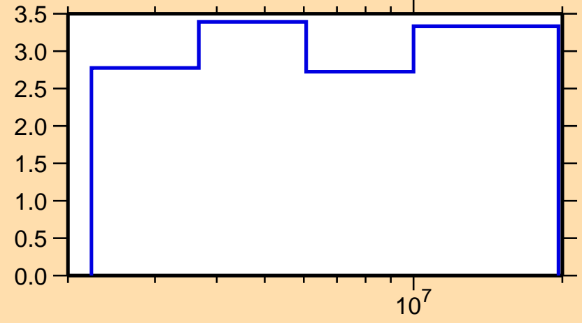
\Delta\sigma/\sigma vs. E for ^{61}\text{Cu}(n,n\text{nonel.})
