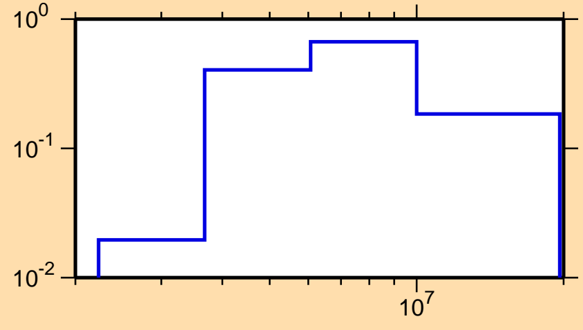
\sigma vs. E for ^{61}\text{Cu}(n,n\text{cont.})
