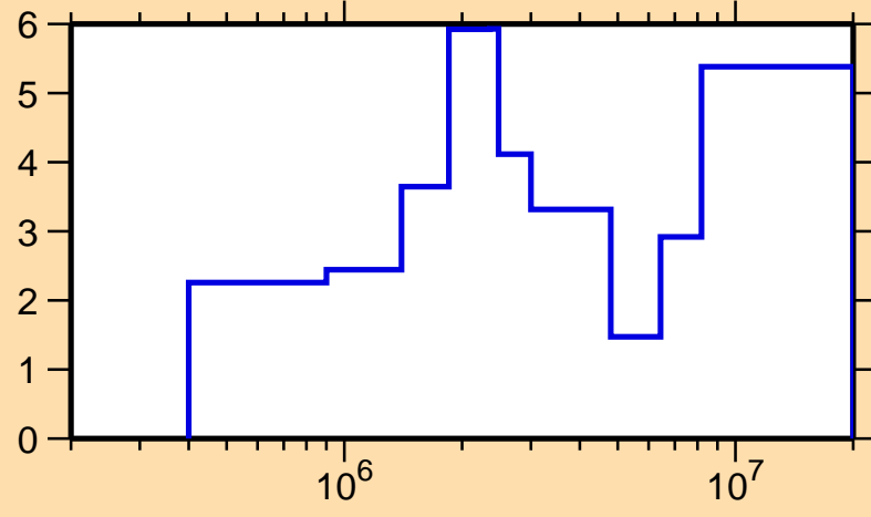
\Delta\sigma/\sigma vs. E for ^{61}\text{Cu}(n,\text{el.})
