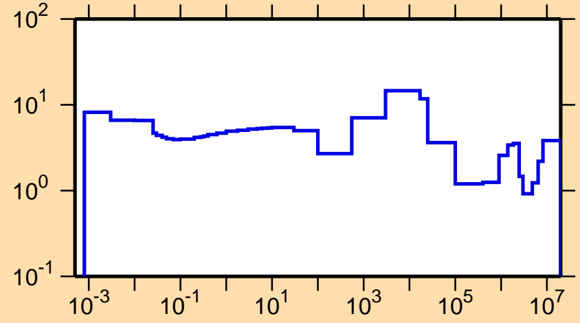
\Delta\sigma/\sigma vs. E for ^{61}\text{Cu}(n,\text{tot.})
