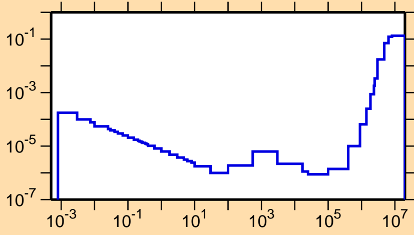
\sigma vs. E for ^{61}\text{Cu}(n,\alpha)
