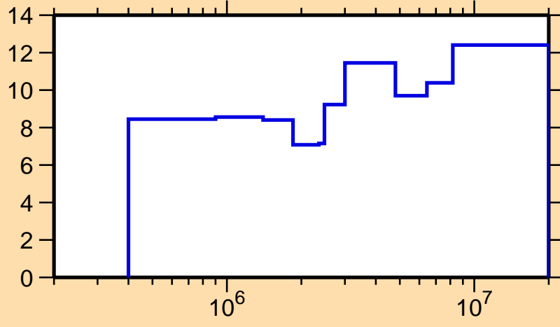
\Delta\sigma/\sigma vs. E for ^{61}\text{Cu}(n,n_1)
