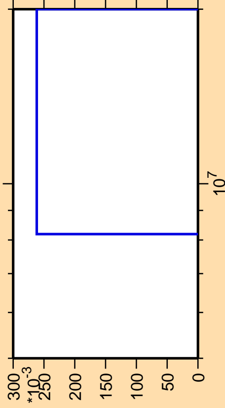
\Delta\sigma/\sigma vs. E for ^{61}\text{Cu}(n,\text{pt})
