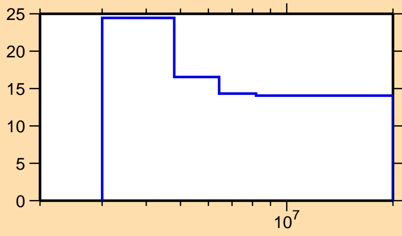
\Delta\sigma/\sigma vs. E for ^{61}\text{Cu}(n,ncont.)
