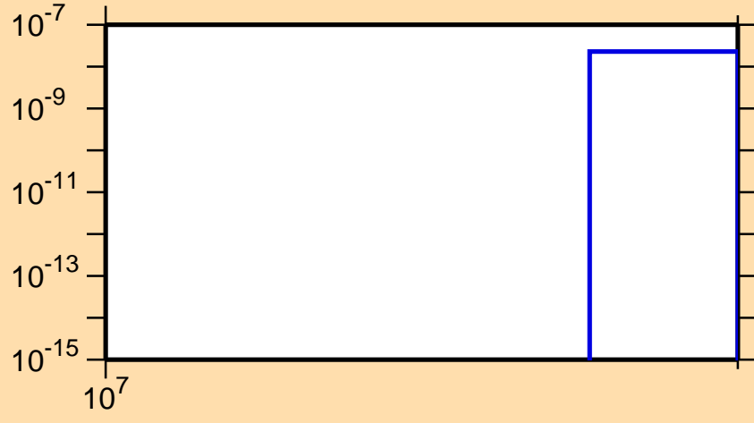
\sigma vs. E for ^{62}\text{Cu}(n,\text{pt})
