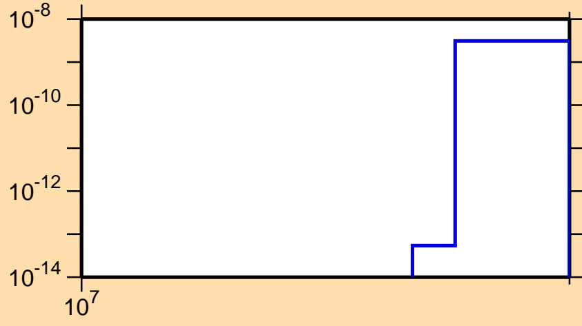
\sigma vs. E for ^{62}\text{Cu} (mt 45)
