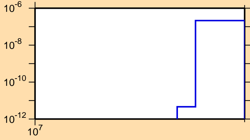
\sigma vs. E for ^{62}\text{Cu}(n,2n\alpha)
