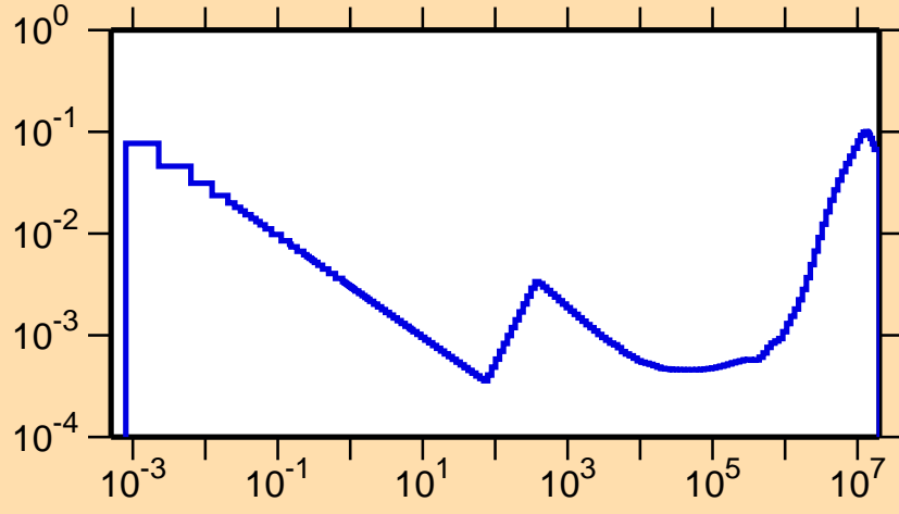
\sigma vs. E for ^{62}\text{Cu}(n,\alpha)
