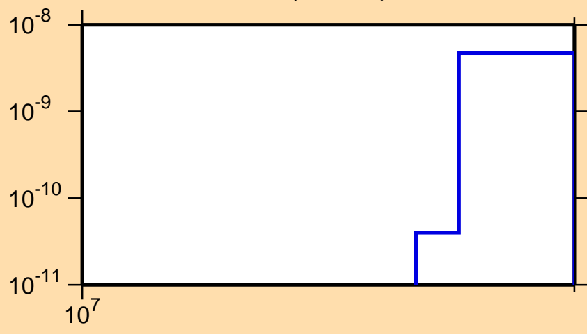
\sigma vs. E for ^{62}\text{Cu}(\text{mt117})
