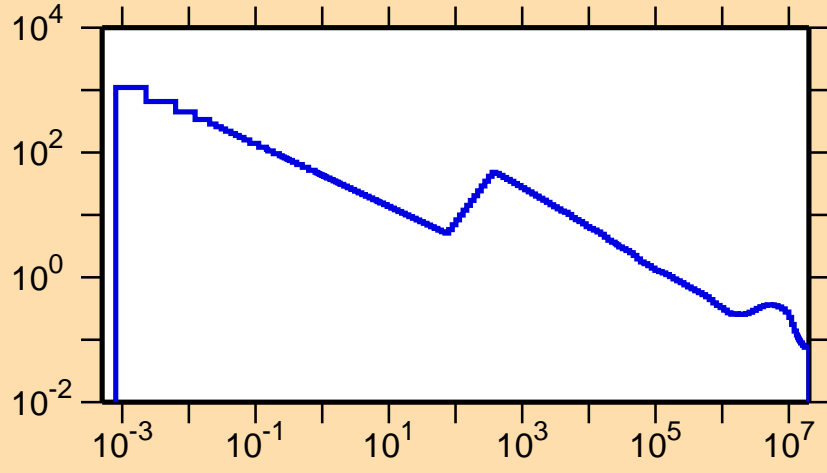
\sigma vs. E for ^{62}\text{Cu}(n,p)
