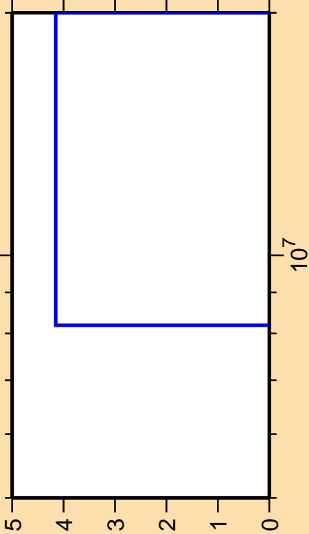
\Delta\sigma/\sigma vs. E for ^{63}\text{Cu}(\text{mt117})
