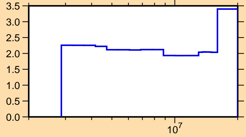
\Delta\sigma/\sigma vs. E for ^{65}\text{Cu}(n,\text{tot.})
