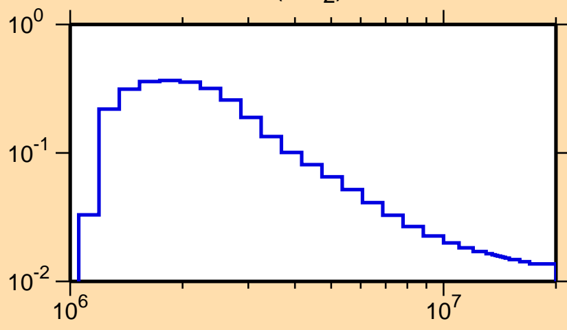
\sigma vs. E for ^{65}\text{Cu}(n,n_2)
