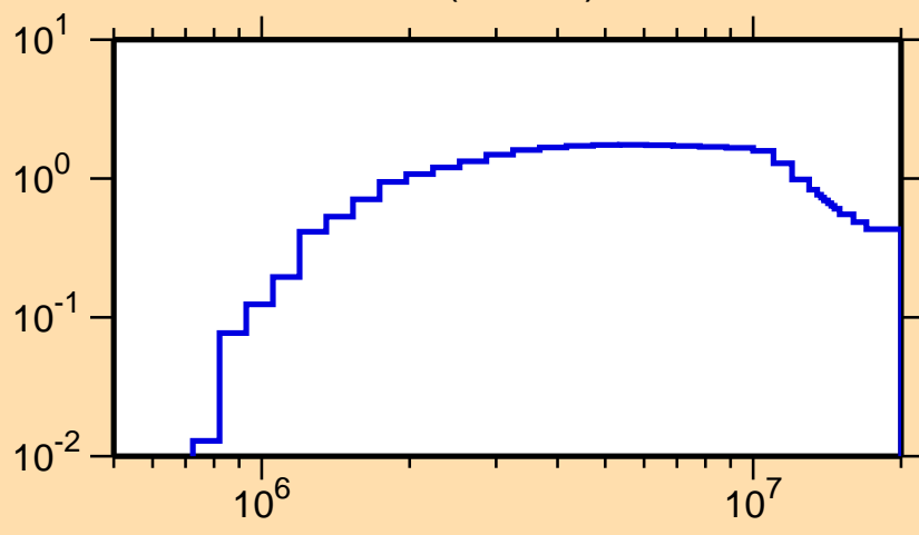
\sigma vs. E for ^{65}\text{Cu}(n,\text{inel.})
