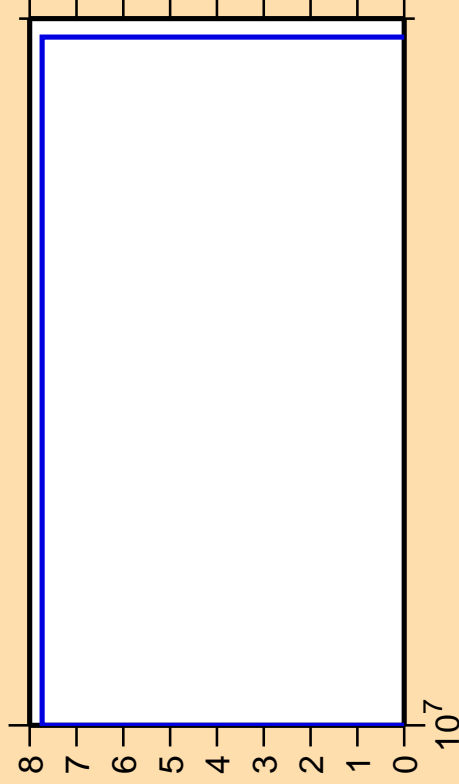
\Delta\sigma/\sigma vs. E for ^{65}\text{Cu}(n,p)
