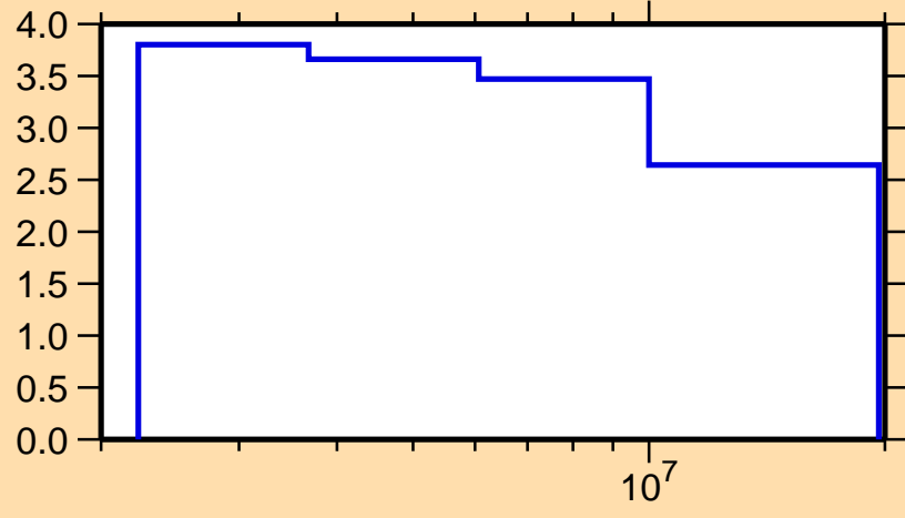
\Delta\sigma/\sigma vs. E for ^{65}\text{Cu}(n,n\text{nonel.})
