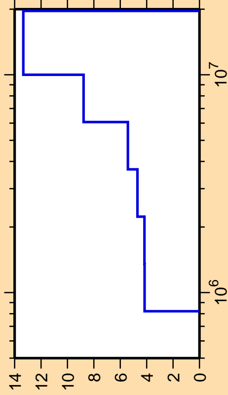
\Delta\sigma/\sigma vs. E for ^{65}\text{Cu}(n,n_2)
