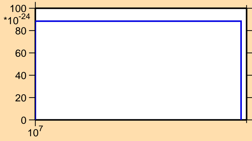
\sigma vs. E for ^{65}\text{Cu}(n,\text{pd})
