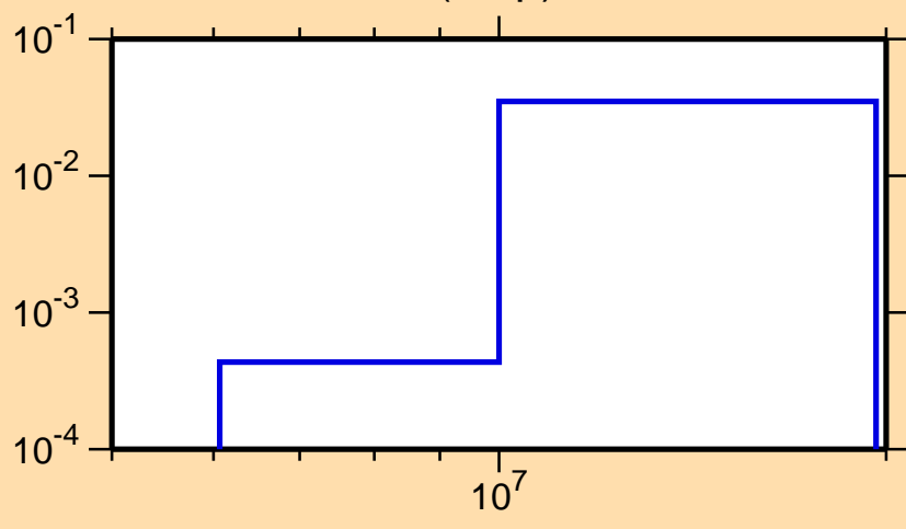
\sigma vs. E for ^{65}\text{Cu}(n,np)
