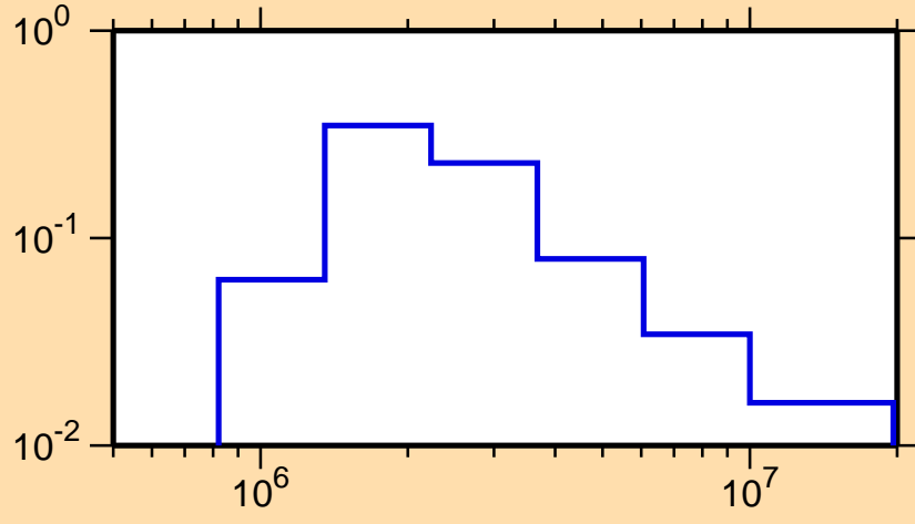
\sigma vs. E for ^{65}\text{Cu}(n,n_2)
