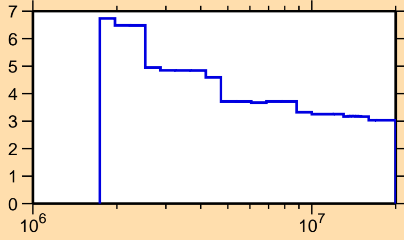
\Delta\sigma/\sigma vs. E for ^{66}\text{Cu}(n,n\text{nonel.})
