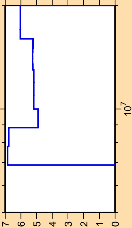
\Delta\sigma/\sigma vs. E for ^{66}\text{Cu}(n,2n)
