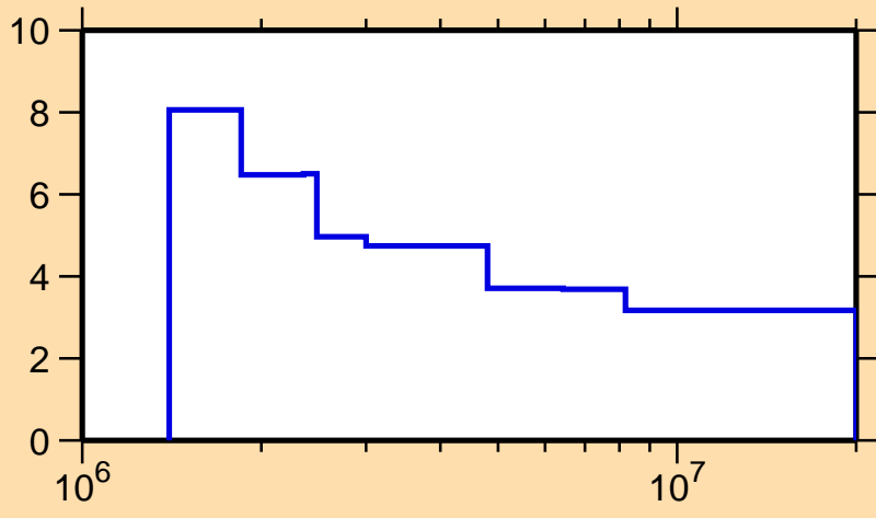
\Delta\sigma/\sigma vs. E for ^{66}\text{Cu}(n,n\text{nonel.})
