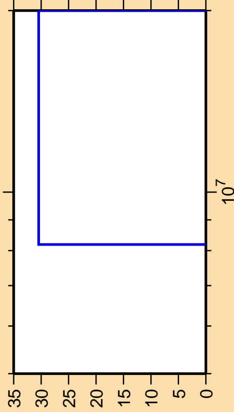
\Delta\sigma/\sigma vs. E for ^{66}\text{Cu}(n,nd)
