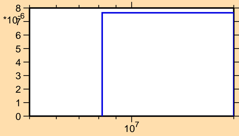
\sigma vs. E for ^{66}\text{Cu}(n,nd)
