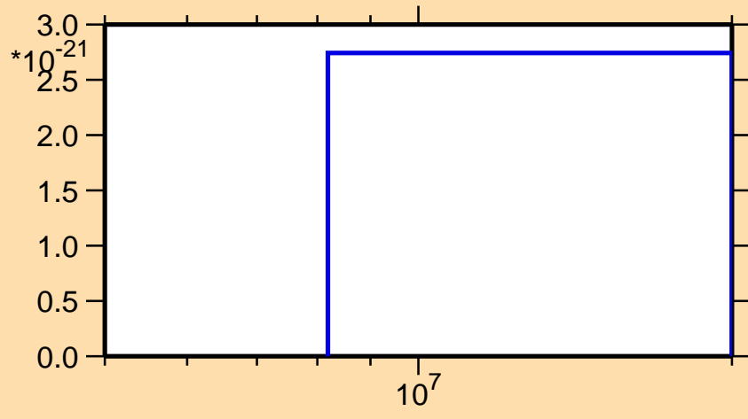
\sigma vs. E for ^{66}\text{Cu} (mt 34)
