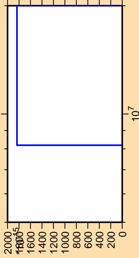
\Delta\sigma/\sigma vs. E for ^{66}\text{Cu}(n,\text{pt})
